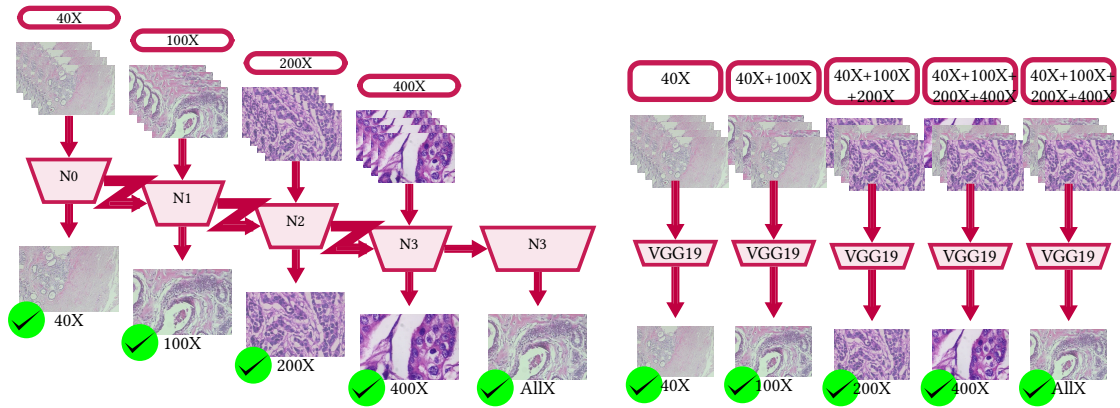
Fig. 3. The INCR approach (on the left) and the CTRL_INCR approach (on the right)
