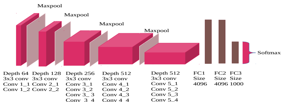
Fig. 2. VGG19 architecture [40], \text{Conv}_i_j are convolutional layers with kernels of size 3 \times 3 , FC1 and FC2 are fully connected layers.
