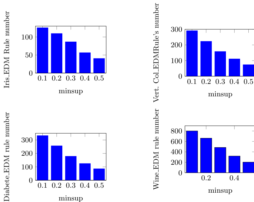
Fig. 1. Generic associative rule’s number for different support values
