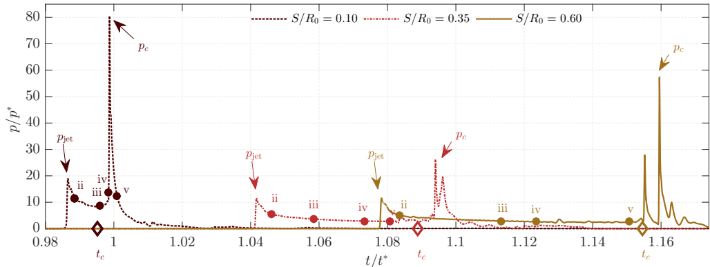
FIGURE 6. Evolution of the wall-centred pressure for the smooth-wall case at varying stand-off distances S/R_0 . The time instances shown in figure 5 are highlighted and labelled with the corresponding row (ii–v). The pressure peaks induced by the jet impact p_{\text{jet}} and the collapse p_c are indicated as such. The collapse time t_c is plotted as a diamond on the x -axis.
