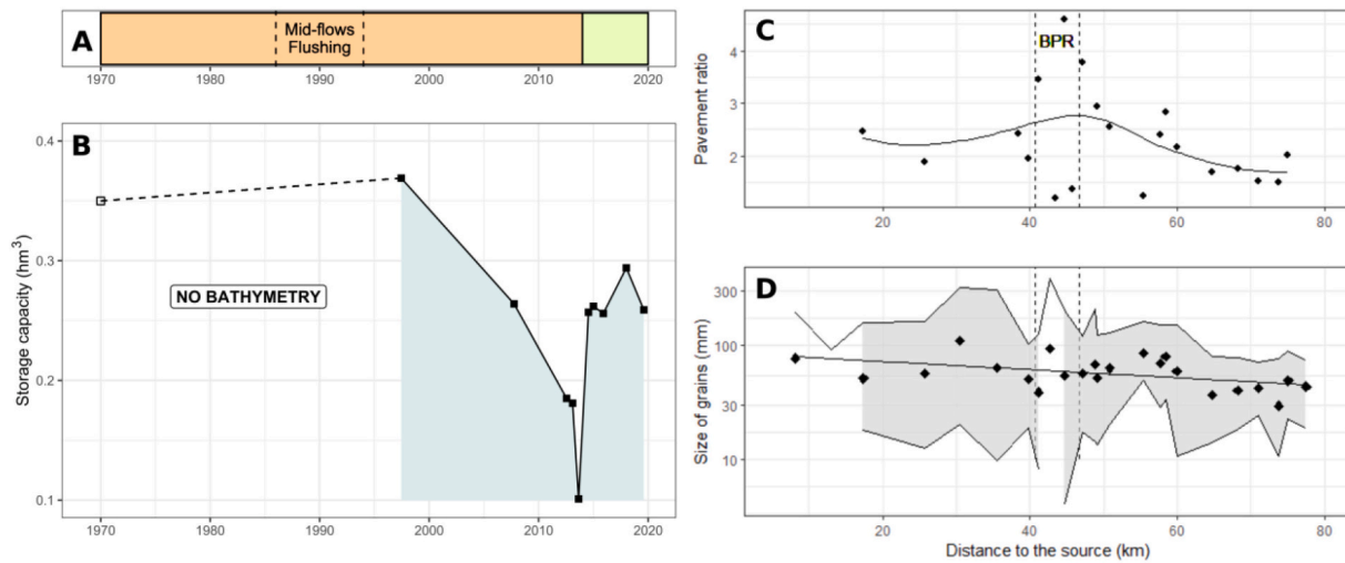
Fig. 7. A) Plan d'Arem dam management. Orange: no drawdown flushing. Green: Drawdown flushing. B) Water storage capacity. C) Longitudinal pattern of armorment ratio. D) Longitudinal pattern of grain size distribution. Black dots: D_{50} . Grey area: D_{10} – D_{90} range. (For interpretation of the references to color in this figure legend, the reader is referred to the web version of this article.)
