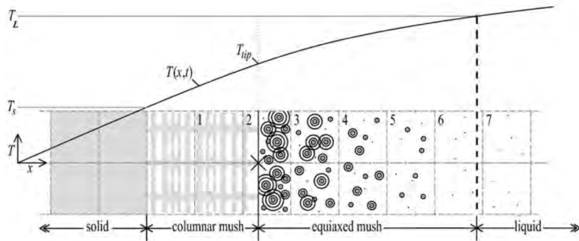
30 Figure 3: Illustration of the concurrent C2ET modelling approach which allows columnar and 31 equiaxed mushy regions to nucleate and grow simultaneously. 32 33 34
