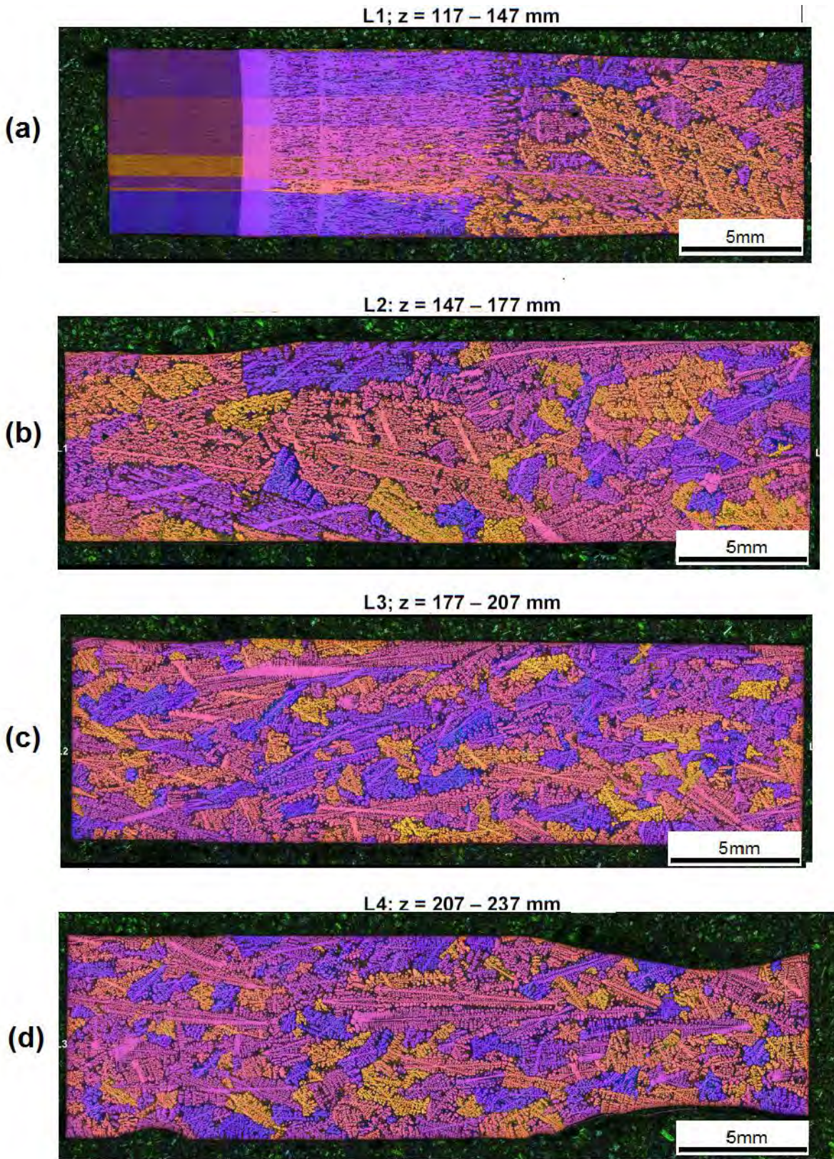
Figure 11: Microstructure image collage for scenario GD#2. Electrolytic etch under a polarising light. Representative axial positions for each micrograph are provided above each image.
