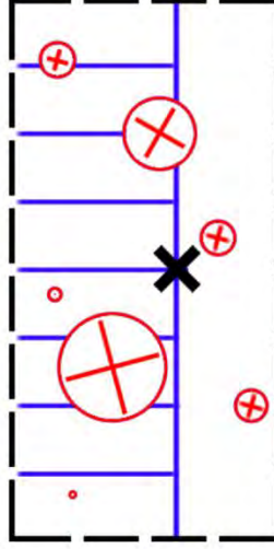
Figure 4: Detailed illustration of a control volume that contains both columnar mush (striped area left of marker \times ) and equiaxed mush (circular crosshairs, \otimes ). Note how an individual equiaxed crystal can exist as phantom growth within the columnar mush or as real growth in the liquid region to the right of the marker.
