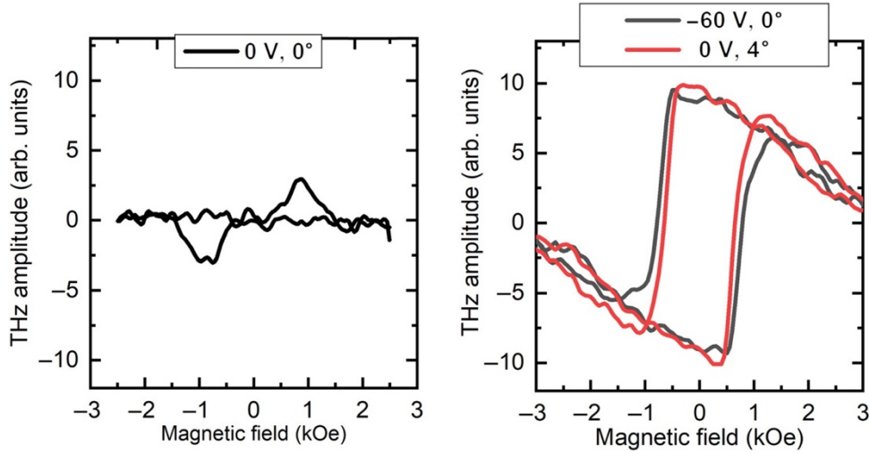
Fig 4. Interchangeability of voltage and azimuthal sample position. Dependences of the maximum THz pulse amplitude on magnetic field for (a) zero voltage and exact hard-axis orientation; (b) two azimuthal sample positions ( 0, 4^\circ ) and two values of applied voltage (0 and -60 V). Delay time is fixed at t=0 ps.
