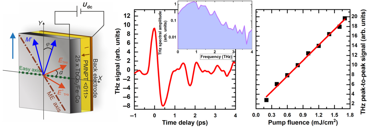
Fig 1. Sample structure and THz pulse characterization. (a) Scheme of the composite multiferroic emitter: orientation of the axes of magnetocrystalline (easy axis) and magnetoelastic (ME axis) anisotropy, external magnetic field \mathbf{H} , magnetization \mathbf{M} , THz-wave electric field \mathbf{E} ; \mathbf{P} , ferroelectric crystal polarization axis normal to the structure plane; \varphi , the angle between magnetization \mathbf{M} and the hard axis ( \varphi = \alpha ). Back electrode is made of copper. (b) Temporal waveform and spectrum (inset) of the generated THz pulse. (c) Dependence of THz peak-to-peak amplitude on the pump fluence.
