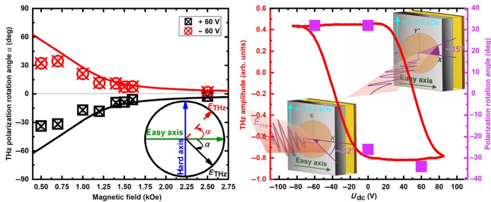
Fig 3. THz polarization rotation (a) \alpha versus magnetic field applied along the hard axis at a substrate voltage of 60, -60 V. Line corresponds to theoretical calculation. Inset, THz polarization angle at two different angular regions relative to the easy axis direction. (b) \alpha versus voltage applied to the substrate at a fixed magnetic field of 0.7 kOe (points, right scale) and corresponding maximum amplitude of the THz pulse (line, left scale).
