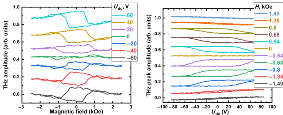
Fig 2. Dependences of the THz amplitude E_y (a) on the magnetic field strength for different voltages and (b) on the voltage for different values of magnetic field strength (THz-amplitude magnetic and electric hysteresis loops, respectively).
