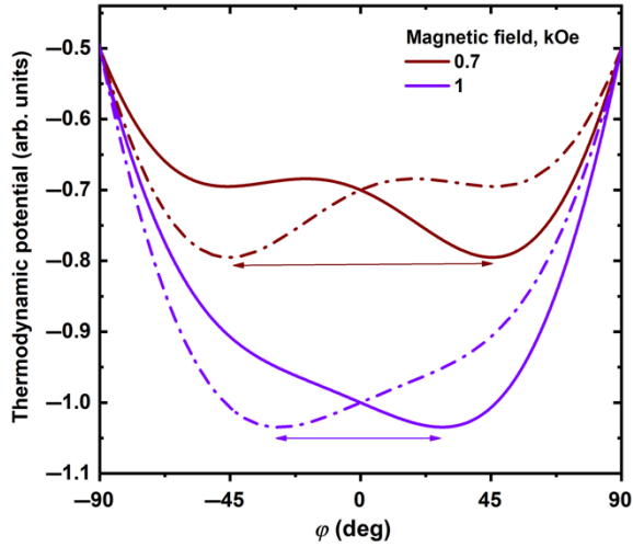
Fig 5. Magnetization switching between two minima. Thermodynamic potential of the magnetic subsystem at a magnetic field strength H=H_A=1 kOe and H=0.7 kOe when applying a voltage of -60 V (solid lines) and +60 V (dashed-dotted lines).
