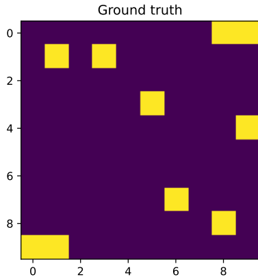
Figure 18: Simulated ground truth. This binary mask locates the simulated signal on a 2D 10 \times 10 grid. Signal locations have been drawn randomly and account for (1 - \pi_0)\% of the image, the rest of the image being null data.
