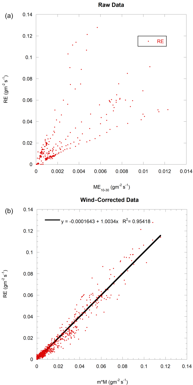
Figure 8. (a) RE versus ME (raw data, average between PWM = 10 and PWM = 30 % measurements). (b) RE versus wind speed corrected ME for all dispoible data along with a linear regression.
