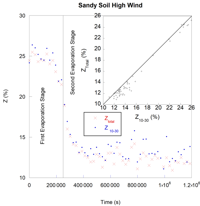
Figure 6. Z_{total} and Z_{10-30} versus time for sandy soil at a relatively strong wind of 1.15 \text{ m s}^{-1} . Insert, the same values of Z_{total} versus Z_{10-30} .
