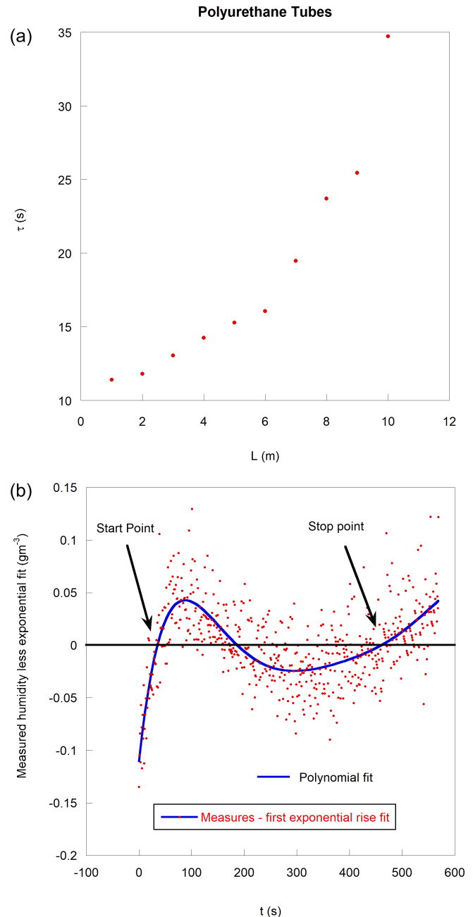
Figure 2. (a) Apparent response time of the polyurethane tubes versus the length of the tubes. (b) Measured absolute humidity less exponential fit (residuals), giving start and stop points for a second regression.
