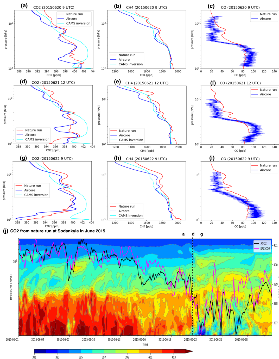
Fig. 5 Examples of CO 2 , CH 4 and CO vertical profiles from the CHE nature run at Sodankylä (67.37°N, 26.63°E). The nature run is compared to NOAA AirCore (v20201223) observations 36,39 and the CAMS CO 2 and CH 4 inversion 57,65,66 (a–i) during three days in June, depicted by the dashed lines in (j) where the nature run hovmöller plot for CO 2 shows the temporal variability of the vertical profile at Sodankylä over the whole month of June. The solid black and magenta lines show the time series of XCO 2 and near-surface CO 2 averaged over the model levels from the surface to 400 m above the surface (SFC CO 2 ) respectively.
