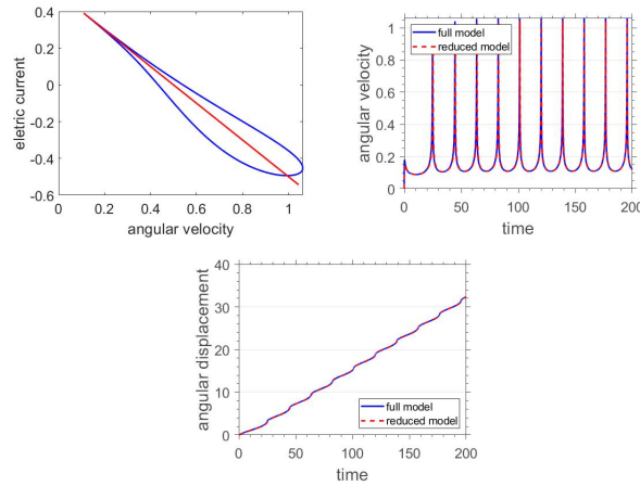
Fig. 8 Phase-space of electric current \hat{q} versus angular velocity \hat{\theta} , angular velocity \hat{\theta} versus t and angular displacement \theta versus t . Dimensionless parameters: \nu = 0.5 , d = 10 , \ell = 0.05 , b = 1 . Initial conditions: (\theta_0, \dot{\theta}_0, \hat{q}_0) = (0, 0, 3\nu)
