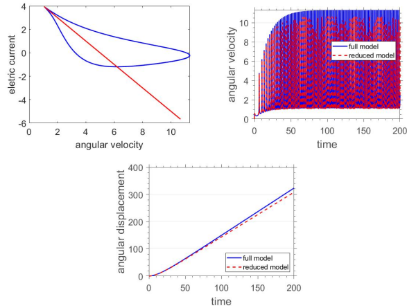
Fig. 9 Phase-space of electric current \dot{q} versus angular velocity \dot{\theta} , angular velocity \dot{\theta} versus t and angular displacement \theta versus t . Dimensionless parameters: \nu = 5 , d = 10 , \ell = 0.05 , b = 1 . Initial conditions: (\theta_0, \dot{\theta}_0, \dot{q}_0) = (0, 0, 3\nu)
