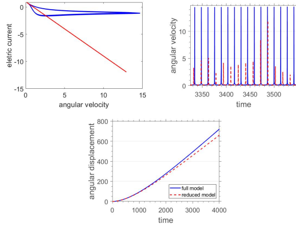
Fig. 7 Phase-space of electric current \hat{q} versus angular velocity \hat{\theta} , angular velocity \hat{\theta} versus t and angular displacement \theta versus t . Dimensionless parameters: d = 100 , \ell = 0.05 , \nu = 1 , b = 1 . Initial conditions: (\theta_0, \dot{\theta}_0, \hat{q}_0) = (0, 0, 3\nu)
