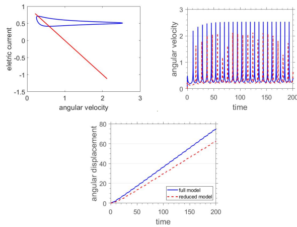
Fig. 4 Phase-space of electric current \dot{q} versus angular velocity \dot{\theta} , angular velocity \dot{\theta} versus t and angular displacement \theta versus t . Dimensionless parameters: \ell = 2, \nu = 1, b = 1, d = 10 . Initial conditions: (\theta_0, \dot{\theta}_0, \dot{q}_0) = (0, 0, 3\nu)
