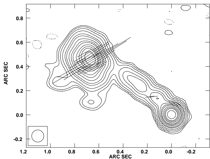
Fig. 3. The MERLIN minus Cambridge (epoch 1995.38) image of 3C 99 at 5 GHz. Contours are at -0.25, 0.25, 0.5, 1, 2, 4, 6, 10, 15, 20, 30, 40, 50, 70, 100 mJy/beam. The peak flux density is 96.4 mJy. The beam is 100 \times 100 mas. An electric field vector length 1'' = 20 mJy/beam.
