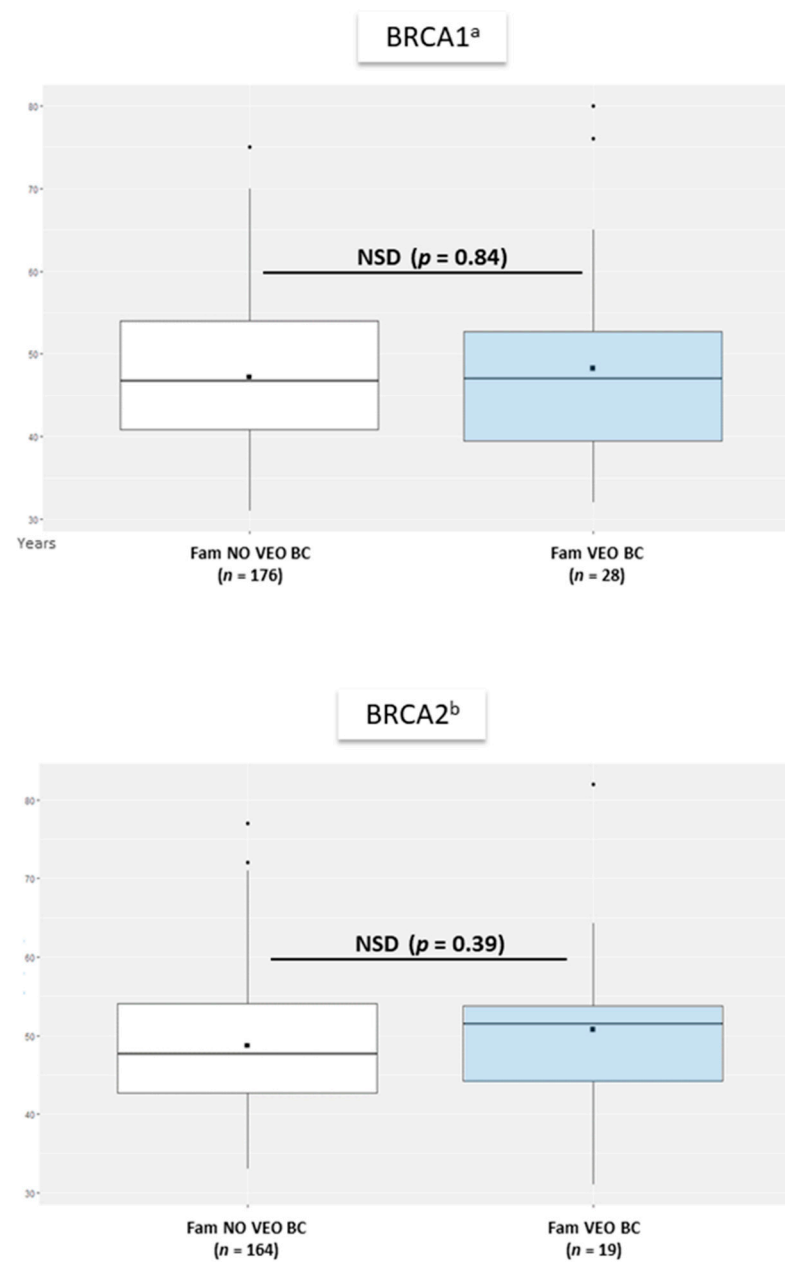
Figure 2. Average of mean age at BC diagnosis in female relatives of women with VEO-BC versus no VEO-BC. a : among BRCA1 mutation ( BRCA1m ) carrier women. b : among BRCA2m carrier women. Fam. VEO-BC: families with at least one VEO-BC. Fam. NO VEO-BC: Families without any VEO-BC. ( n ): number of families with available data for age at first BC diagnosis in women. NSD: nonsignificant difference (two-sided Wilcoxon–Mann–Withney test). Horizontal line is median, box edges are 1st and 3rd quartile and whiskers are range of age at diagnosis of BC in relatives in each family. Central black square is the mean average age at diagnosis of BC in relatives in each family.
