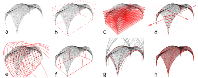
Figure 2: Main steps in the reverse engineering process of a groin vault.
