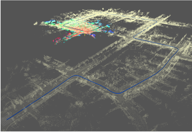
Fig. 6. The mapping result of the proposed Lidar registration algorithm using first 125s of the KITTI dataset kitti_2011_10_03_drive_0027_synced [62]. The blue line denotes the vehicle trajectory. The blue and green points denotes the local map while red points denotes the matching result. The white points represent the reconstructed dense map after covariance-aided pose graph optimization.
