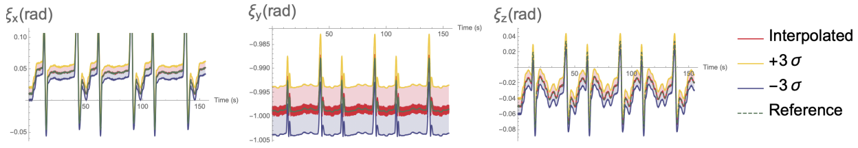
Fig. 4. The interpolated results and their 3\sigma bounds for the eigenaxis \xi .
