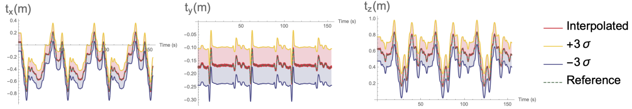
Fig. 5. The interpolated results and their 3\sigma bounds for the translation t .
