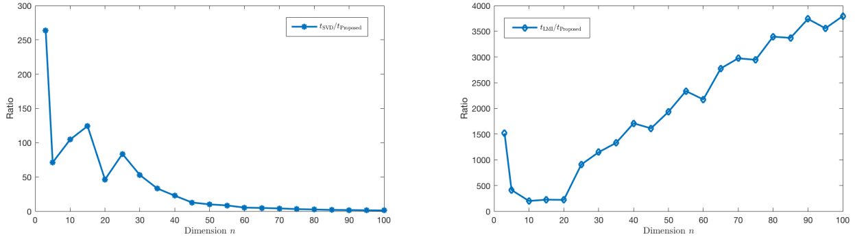
Fig. 2. The ratios of computation time from SVD, LMI and the proposed method.
