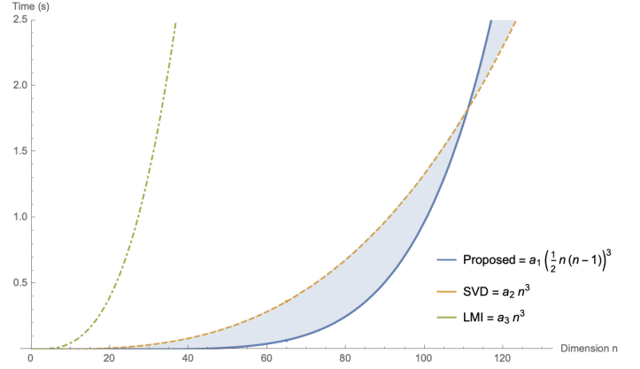
Fig. 1. Time complexity performances of various algorithms.
