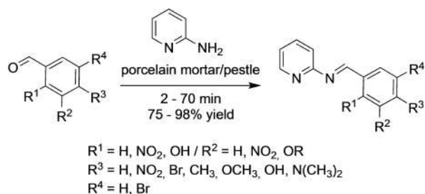
Scheme 11. Mechanochemically synthesized azomethine derived from 2-aminopyridine.
