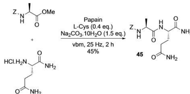
Scheme 50. Mechanoenzymatic peptide coupling.
