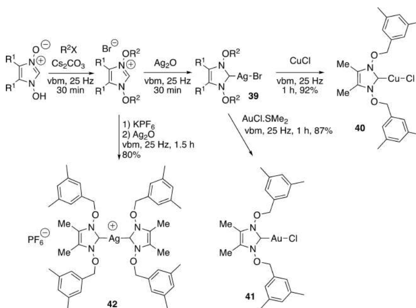
Scheme 42. Mechanosynthesis of novel NOHC-metal complexes.
