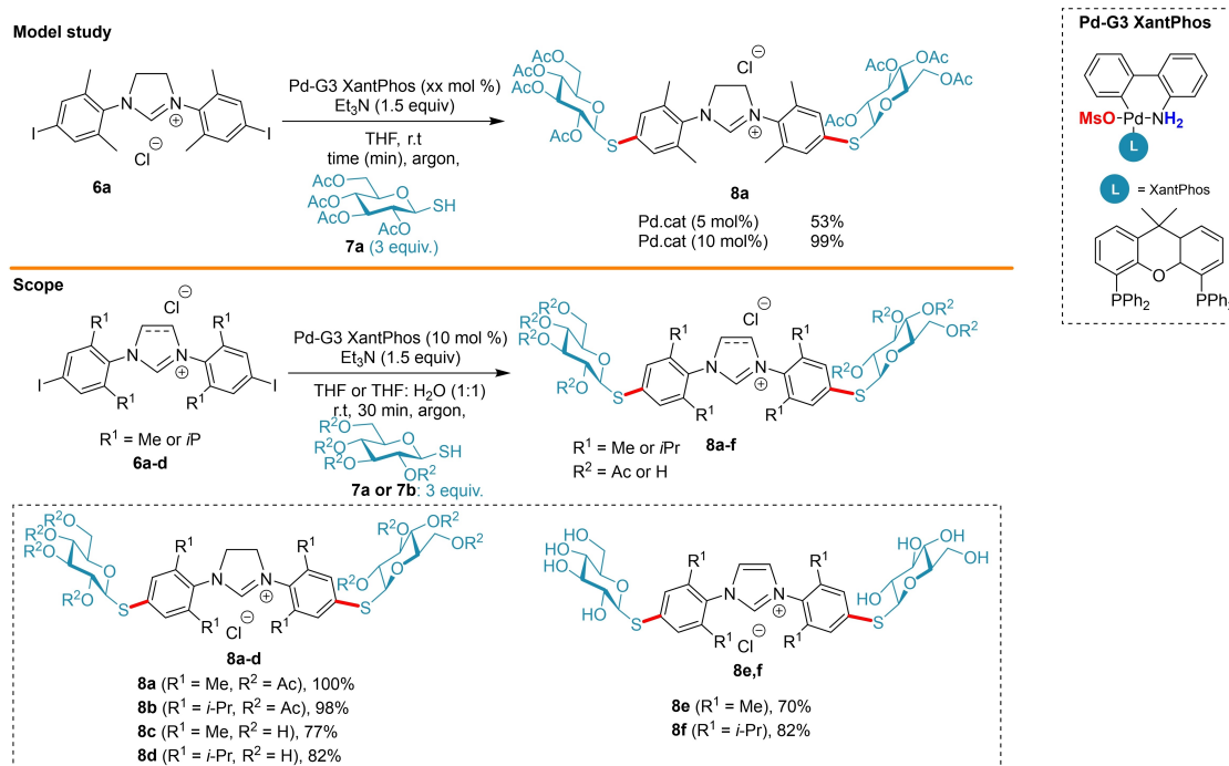
Scheme 1. Coupling of various imidazolium and imidazolium 6a–d with thiosugars 7a–b .
