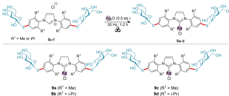
Scheme 2. Preparation of NHC–Ag(I)-thioglycosides 9a–d using vibratory ball mill approach. Reaction conditions: 8c–f , Ag 2 O (0.5 equiv.), 10 mL stainless steel jar, 1 cm diameter stainless steel ball, vibratory ball-mill, 30 Hz, 1–2 h.
