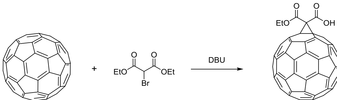
Scheme 1. The Bingel reaction.
