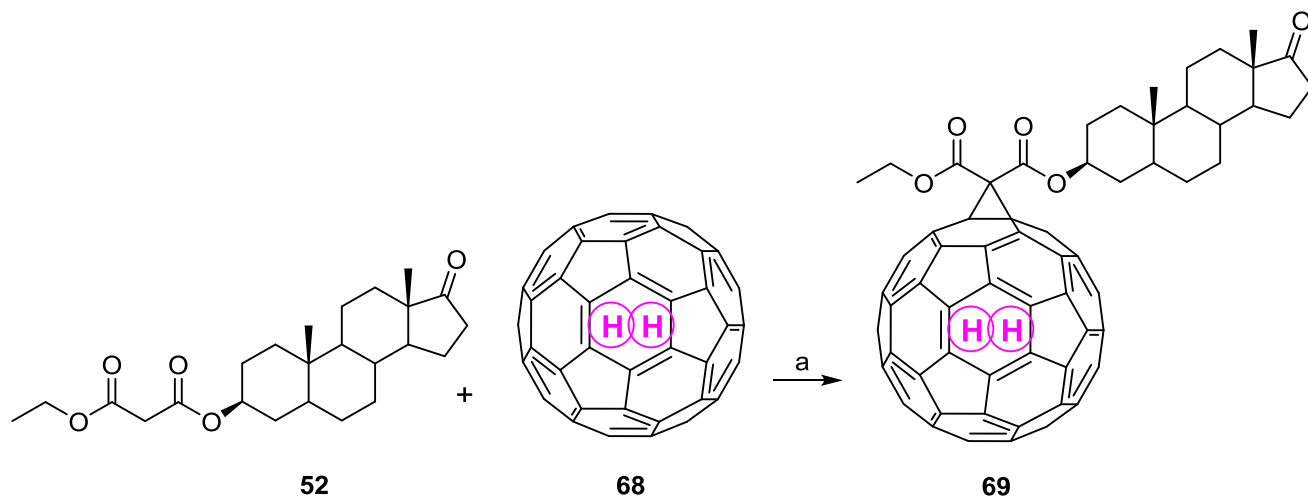
Scheme 16. Synthesis of steroid-fullerene hybrid 69 .
