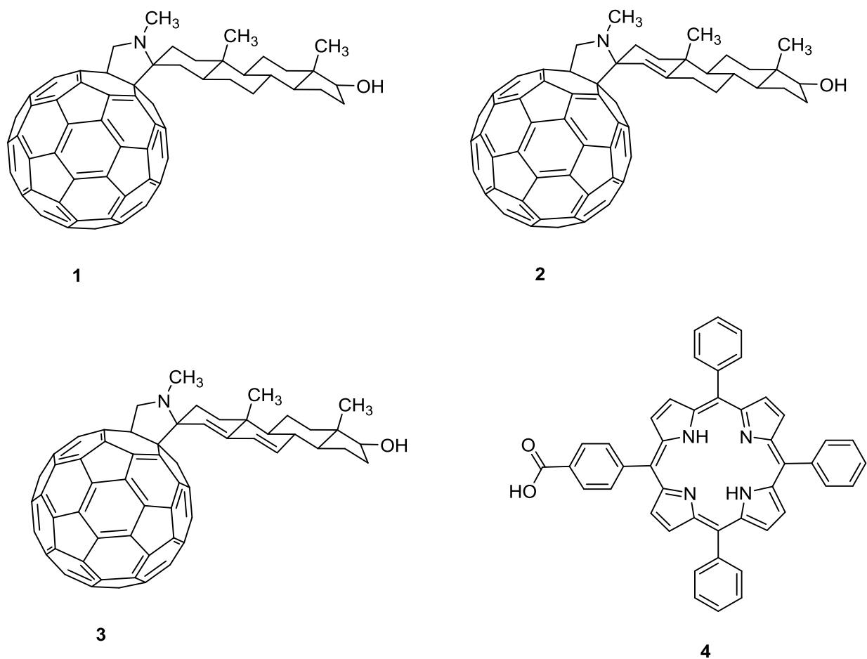
Figure 1. Synthesis of steroidal fulleropyrrolidine precursors 1 , 2 , and 3 and the tetraphenylporphyrin carboxylic acid 4 .
