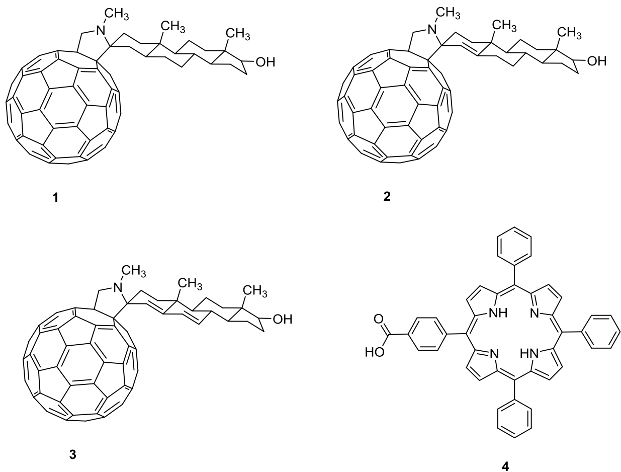
Figure 1. Synthesis of steroidal fulleropyrrolidine precursors 1 , 2 , and 3 and the tetraphenylporphyrin carboxylic acid 4 .
