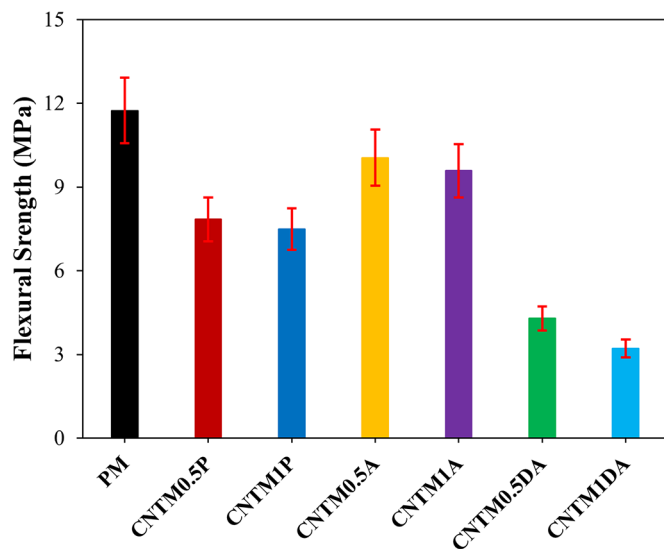
Fig. 15. Flexural strength of cementitious composites after 28-days.
