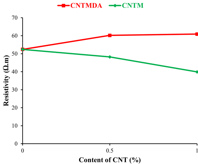
Fig. 7. Resistivity versus content of CNT after 28 days of curing.
