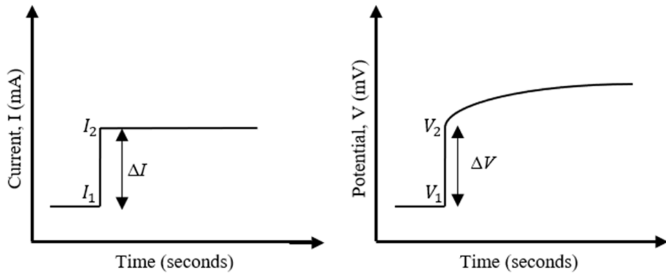
Fig. 3. Schematic view of galvanostatic pulse technique.
