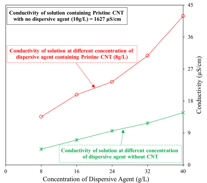
Fig. 9. Conductivity of solutions containing CNTs at various concentrations of dispersive agent.
