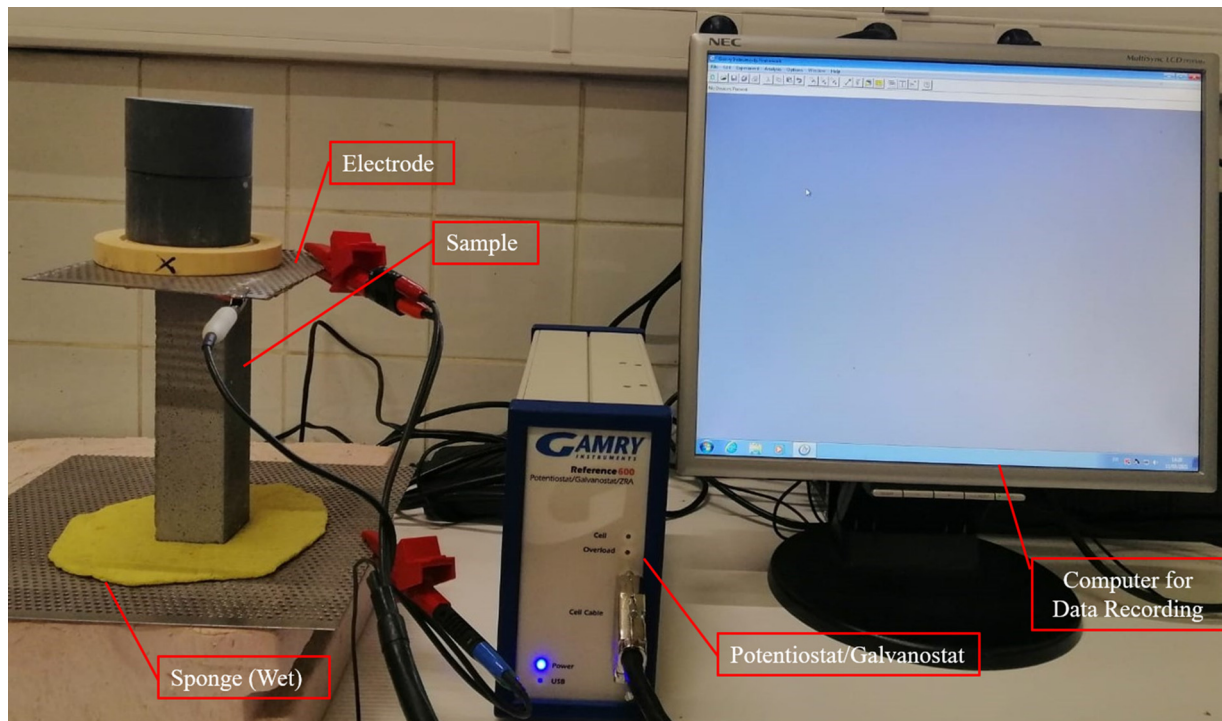
Fig. 2. Setup for resistivity test.
