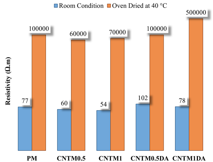
Fig. 8. Resistivity values of specimens after 3 weeks under different saturation conditions.
