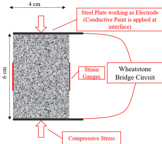
Fig. 5. Schematic representation of test setup.
