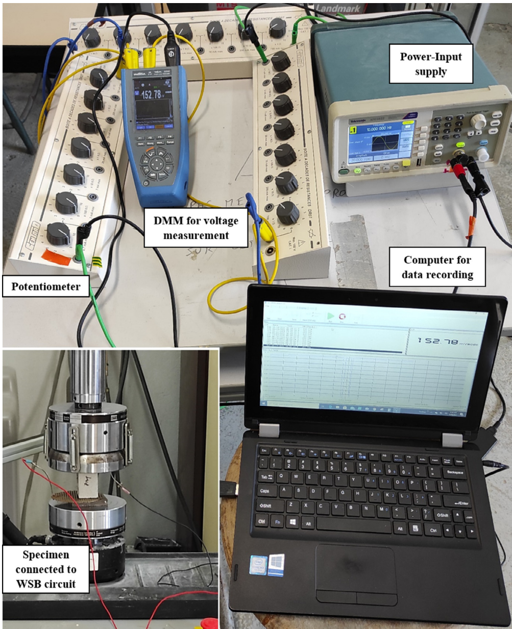
Fig. 4. Wheatstone bridge circuit setup for sensing test.
