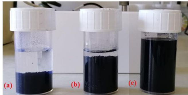
Fig. 1. Suspension of CNT in water after 3 months of preparation of solution: (a) pristine CNT (0.2 g/20 mL), (b) annealed CNT (0.2 g/20 mL), and (c) CNT with 0.2 g of dispersive agent (0.2 g/25 mL).
