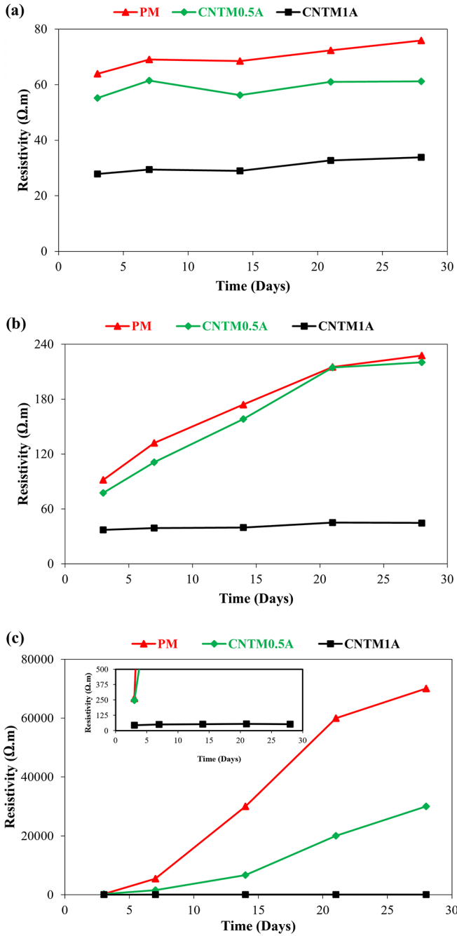
Fig. 12. Resistivity of specimens under (a) saturated surface dry (SSD) conditions, (b) room conditions (RC) and (c) oven dried (OD) conditions.
