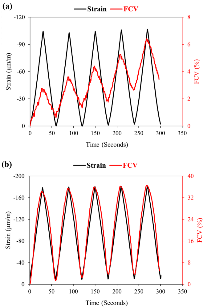
Fig. 17. Piezo-resistive response of (a) PM and (b) CNTM1A under cyclic loading.
