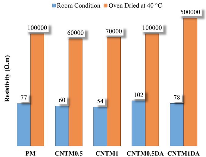
Fig. 8. Resistivity values of specimens after 3 weeks under different saturation conditions.
