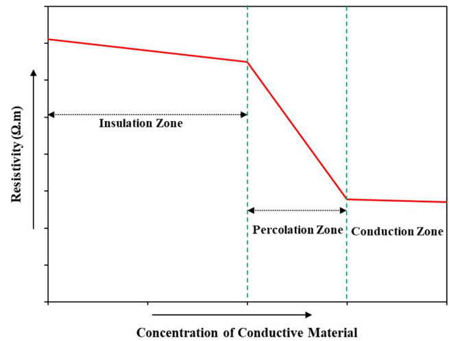
Fig. 11. Schematic representation of various conductive zones.
