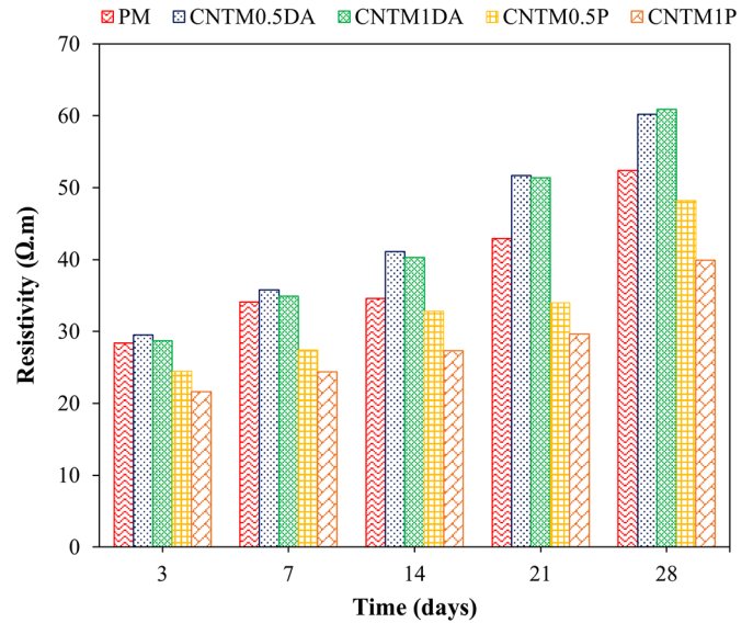
Fig. 6. Resistivity values of saturated specimens after various curing times for plain mortar and mortar with 0.5 and 1% dosage of CNT.
