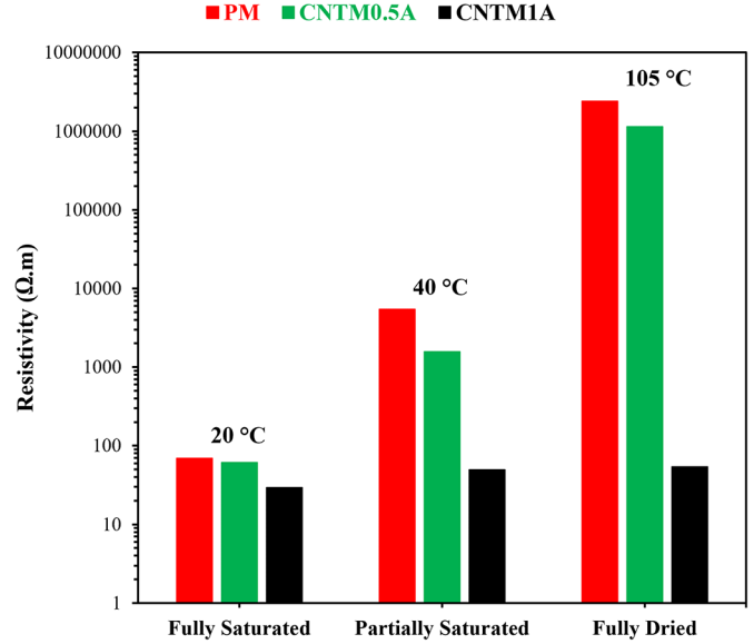
Fig. 13. Resistivity of specimens at different degree of saturation.
