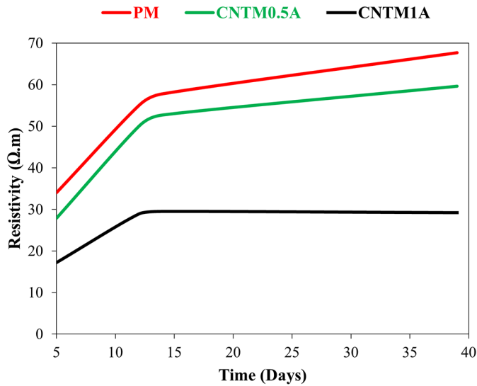
Fig. 10. Evolution of resistivity with curing period for plain mortar and mortar reinforced with 0.5% and 1% of annealed CNT.
