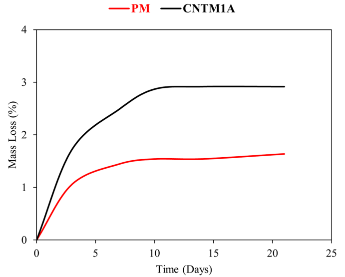
Fig. 16. Mass loss versus time under controlled atmosphere (20 °C and RH 50%).
