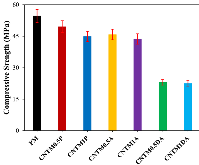
Fig. 14. Compressive strength of cementitious composites after 28-days.
