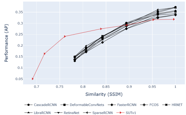
Figure 2: Comparison between the SUT and the baseline models against Gaussian blur.
