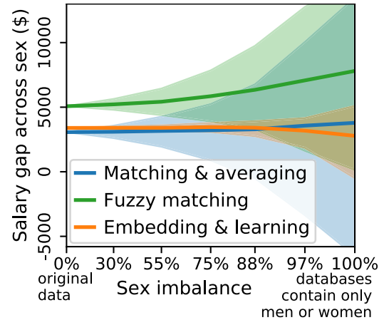
FIGURE 4. Salary gap: Average treatment effect computed with added sex imbalance in individual databases, forcing the need for analysis across databases. The error bars give the quantiles across random deletion of men or women records.
