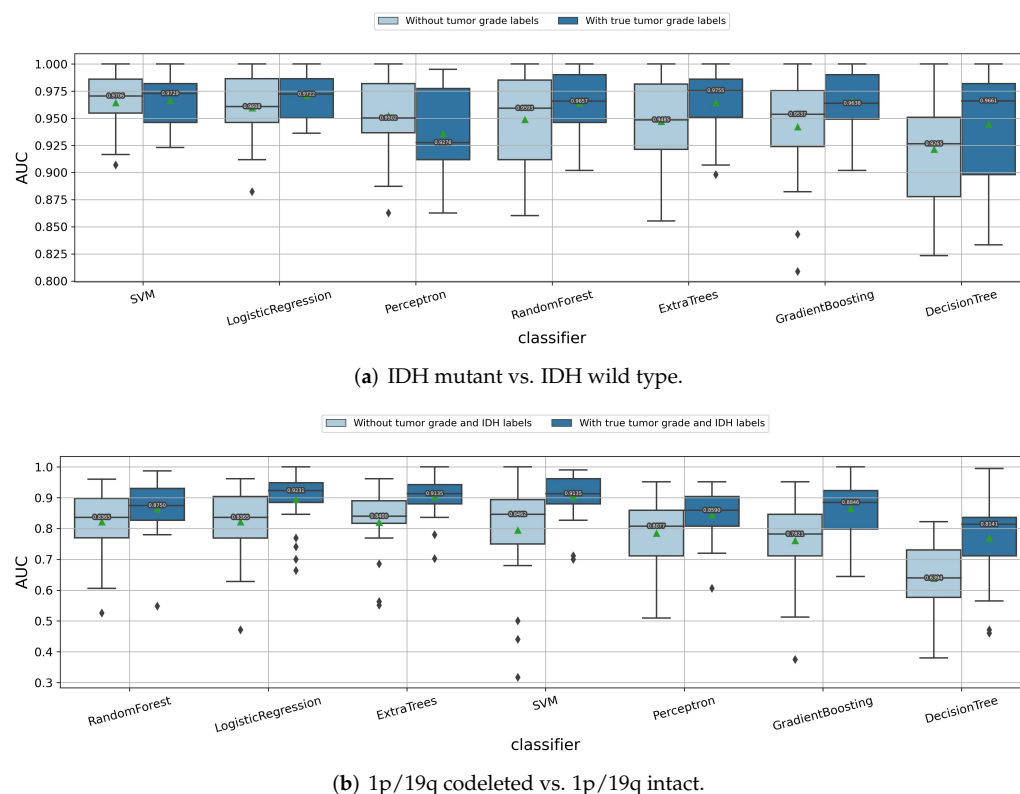
Figure 9. Comparison of whether it helps to improve the performances by using the classifier chain idea, with the true labels of previous classifiers given. (a) Predicting IDH mutation status of the gliomas; (b) predicting 1p/19q codeletion status of the gliomas.
