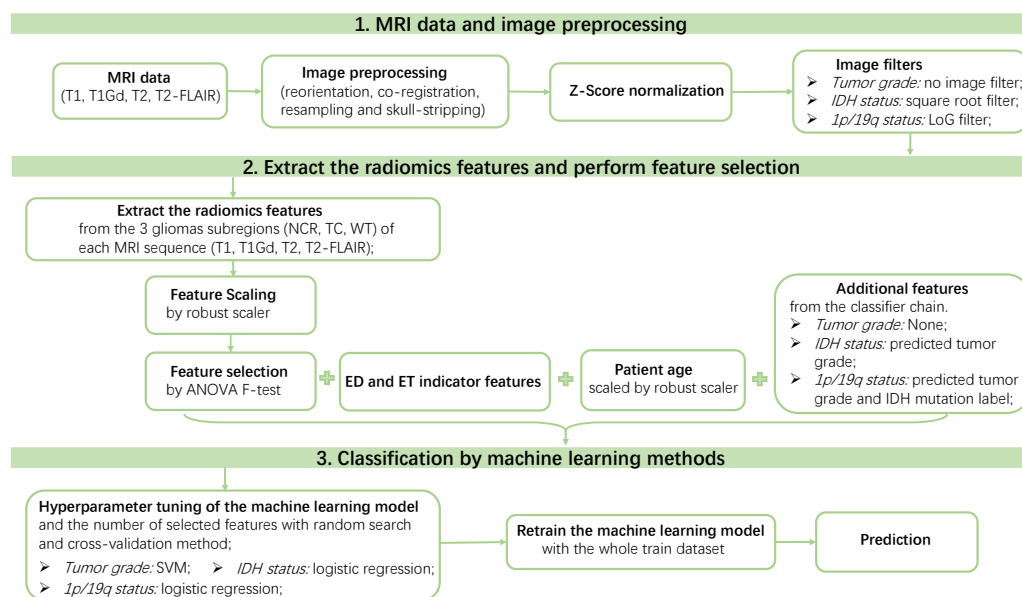
Figure 11. Final radiomics pipeline for predicting each binary classification label (tumor grade, IDH mutation status, and 1p/19q codeletion status) of the gliomas tumor. During the hyperparameter tuning process, the mean cross-validation AUC is used as the evaluation metric.
