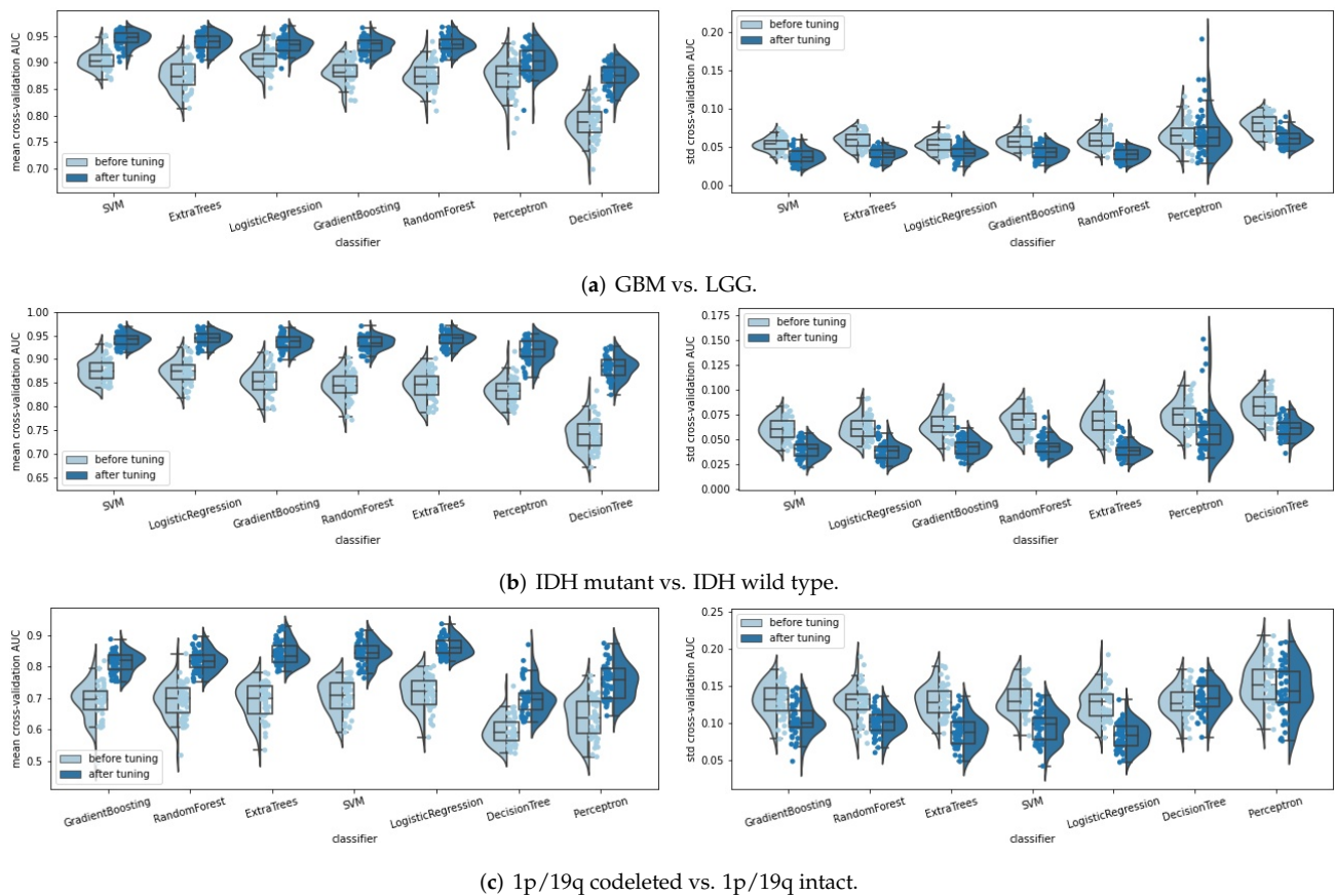
Figure 10. Distribution (displayed by violin plot, box plot, and strip plot) of the mean and STD cross-validation AUC values before and after the pipeline tuning process, for predicting (a) the tumor grade, (b) IDH mutation status, and (c) 1p/19q codeletion status of the gliomas. Each reported point corresponds to a sample random run within 51 random seeds.
