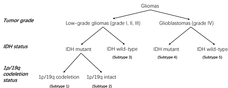
Figure 1. Classification of the glioma tumors used in this paper. This is a simplified version of the classification criteria of gliomas from the 2016 CNS WHO [2]. The subtype numbers 1 to 5 represent the five different glioma subtypes. They can be summarized, respectively, as subtypes “1—LGG, IDH mutant, 1p/19q codeleted”, “2—LGG, IDH mutant, 1p/19q intact”, “3—LGG, IDH wild type”, “4—GBM, IDH mutant”, and “5—GBM, IDH wild type”.
