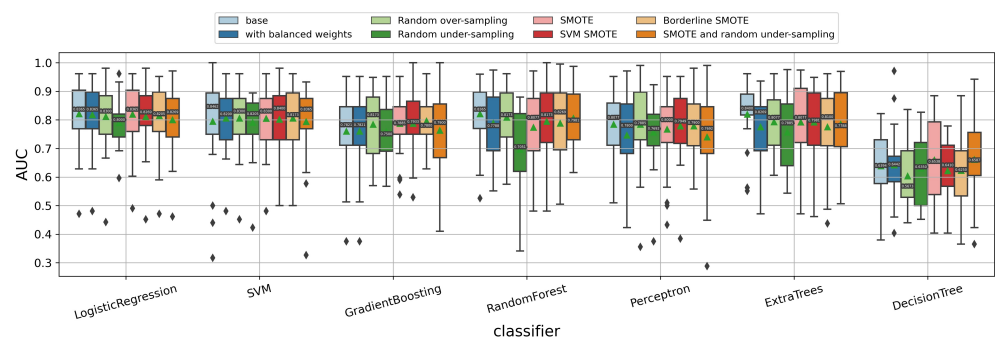
Figure 8. Impact of further data imbalance strategies on predicting the 1p/19q codeletion status of the gliomas. Here, the possible regularization was already applied for each classifier, so “base” means not further using any other data imbalance strategies. “SMOTE and random under-sampling” represents the combination of SMOTE and random under-sampling method.
