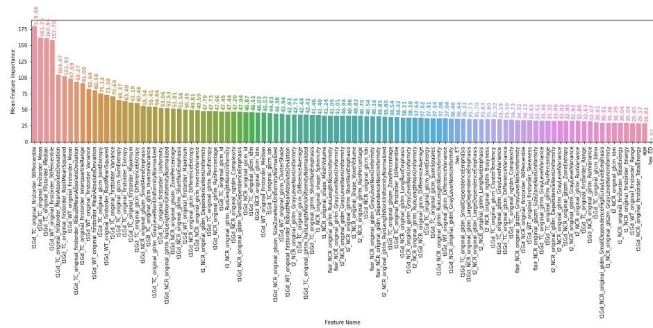
(a) GBM vs. LGG
