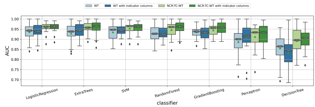
(a) GBM vs. LGG.
