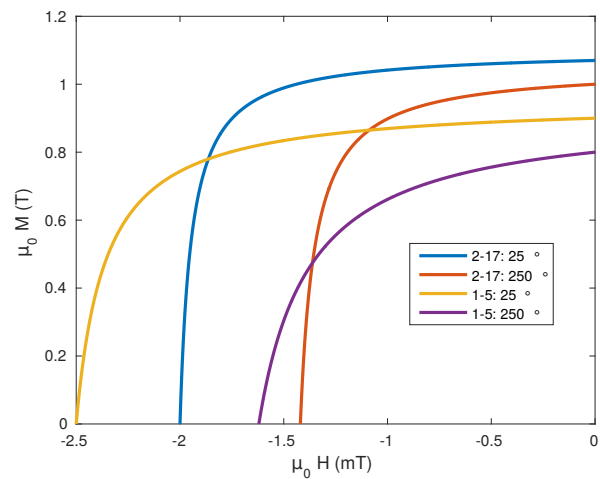
Fig. 6. Demagnetization curves of Sm_2Co_{17} and SmCo_5 at room temperature and 250^\circ\text{C}
