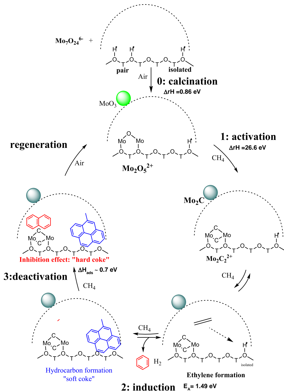
Scheme 6. Mechanisms involved in the four steps of the methane dehydroaromatization reaction.
