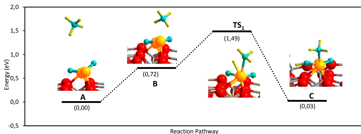
Figure 4: Reaction mechanism for diffusion into zeolite and activation of the first \text{CH}_4 for the catalytic MDA reaction on [\text{Mo}_2\text{C}_2]^{2+} system at 700\text{ }^\circ\text{C}
