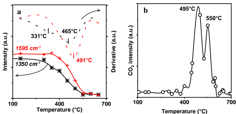
Figure 11: (a) Analysis of both 1350 (black) and 1595 cm -1 (red) Raman peaks - typical of polyaromatic hydrocarbons- recorded along the TPO of the spent catalyst Sp/2.04: evolution of peak area as a function of temperature (plain lines) and corresponding derivative (dot-dashed lines). (b) CO 2 production measured online -simultaneously to the collection of Raman spectra shown in (a). The lines are drawn simply to guide the eyes
