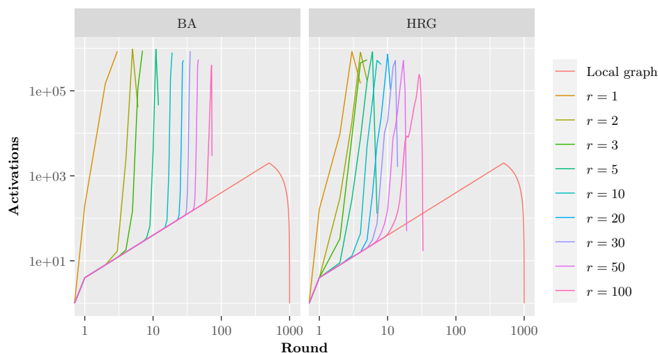
Fig. 2: The number of new active nodes in every round for different configurations. All runs are on n = 10^6 nodes with one initially active node. In one run (“Local graph”), we only consider the 2-dimensional torus on n nodes, while all other runs are on both the torus and a Barabási–Albert random graph (left), or hyperbolic random graph (right). Note that both axes are logarithmic.
