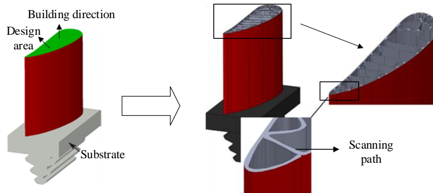
Fig. 10 The redesign of an engine blade based on scanning path [51]. Adapted with permission. wiring and it is redesigned to fulfill the objectives of weight reduction [50] (see Fig. 9). Actually, from the perspective of life-cycle product management, AM enables the real integration of design and manufacturing [52]. For the purpose of functionality and manufacturability integration, the structural optimization of a blade [51] by taking into consideration of manufacturing path and load condition is illustrated in Fig. 10.
