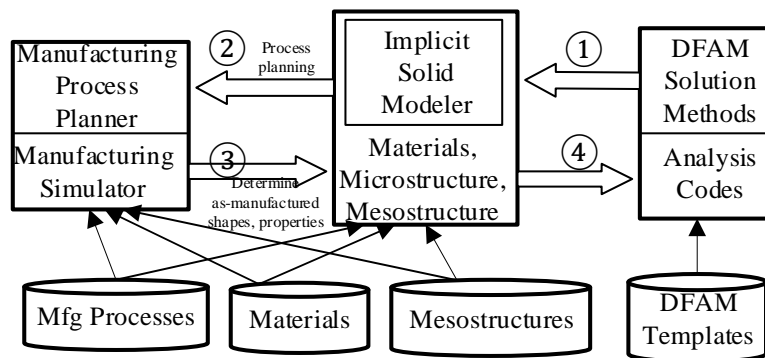
Fig. 16 DFMA system and overall methods [96]. Adapted with permission.
