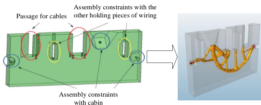
Fig. 9 The redesign of a cockpit plane for weight reduction [50]. Adapted with permission.
