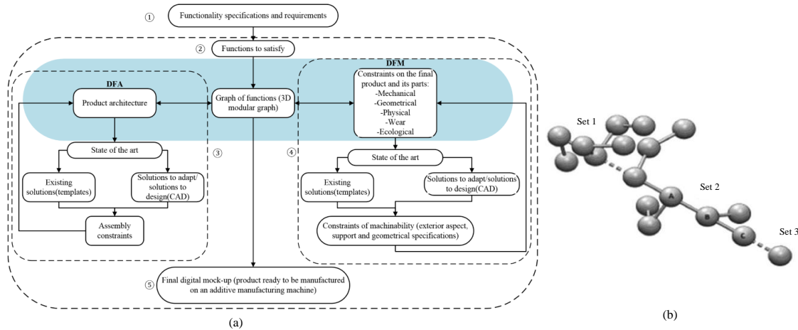
Fig. 13 Design methodology proposed by Boyard and Rivette [63]: (a) the modified DFMA method; (b) function graph.
