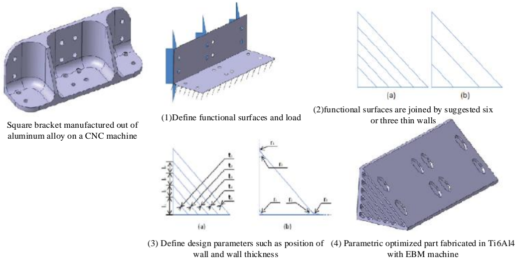
Fig. 15 The redesign process of a square bracket modified from [94].
