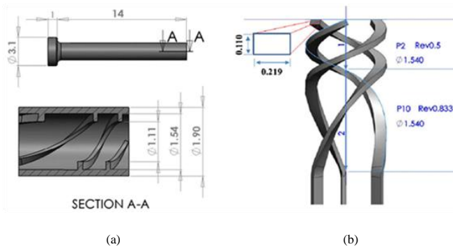
Fig. 4 3D model of the sleeve with micro-vane: (a) hollow tube and section, (b) microvanes (dimensions in mm) [35]. Adapted with permission.
