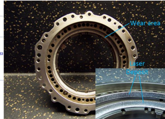
Fig. 5 Low-wattage repair of Ti-6AL-4V bearing housing [36]. Adapted with permission.
