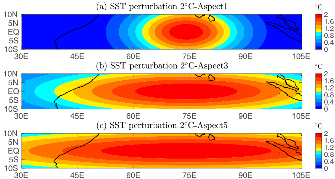
FIG. 3. The SST perturbations (colors, °C) used in the (a) Aspect 1, (b) Aspect3, and (c) Aspect5 experiments with a 2°C maximum amplitude.
