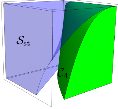
(a) \mathcal{S}_{\text{st}} and \mathcal{C}_4 from Example 5.
