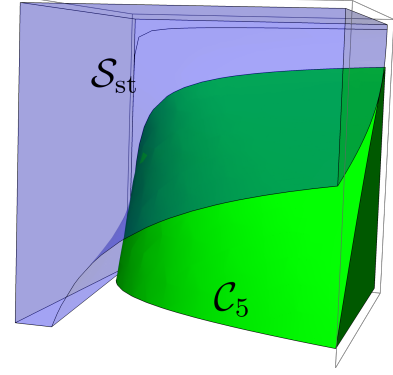
(b) \mathcal{S}_{\text{st}} and \mathcal{C}_5 from Example 6.
