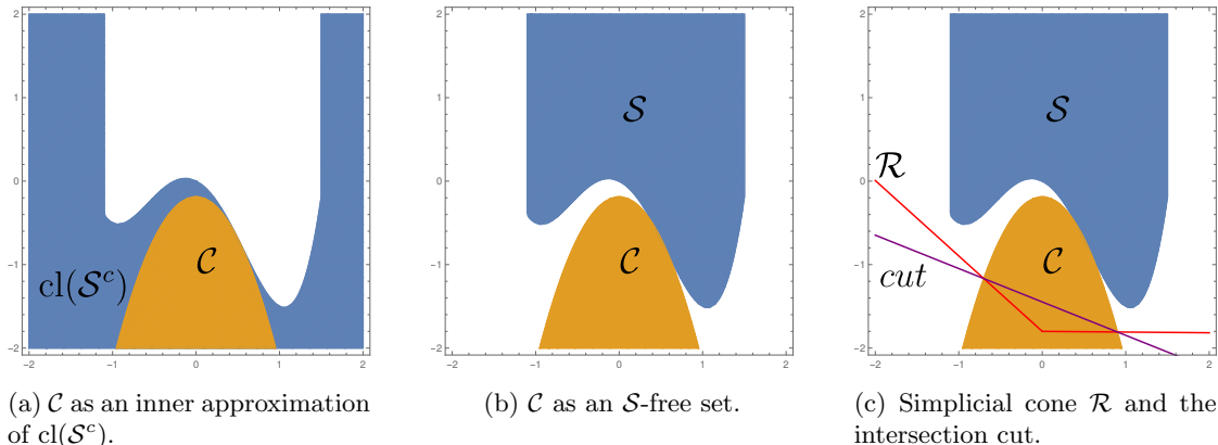
Figure 1: An \mathcal{S} -free set \mathcal{C} , simplicial cone \mathcal{R} , and intersection cut.
