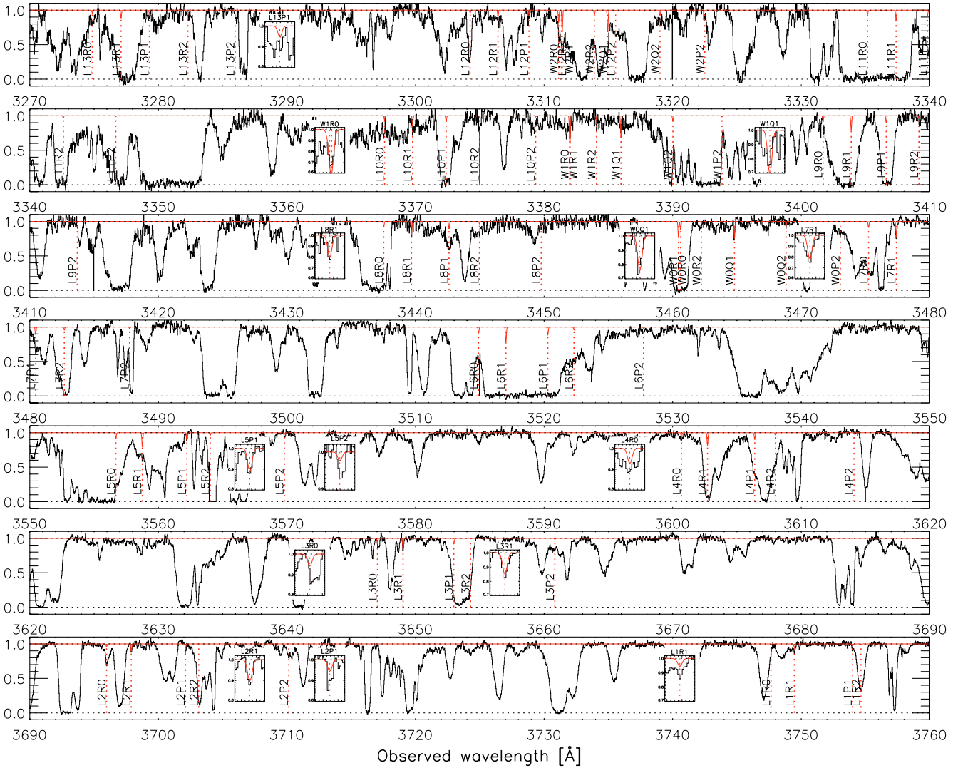
Fig. 2. Portion of the normalized spectrum of Q 2343+125. The resolving power is R \approx 45\,000 . The best fit to the H 2 lines is superimposed on the spectrum. Transition names are written AxBz , with A = L or W for the Lyman or Werner band systems; x is the quantum number of the vibrational upper state, while B is the branch designation ( P , Q or R for \Delta J = +1 , 0 , -1 respectively) and z is the rotational quantum number of the lower state. The fit parameters are given in Table 1. Zooms into individual lines are shown in small boxes that are shifted horizontally for clarity. Each box is 0.5 \text{ \AA} wide.
