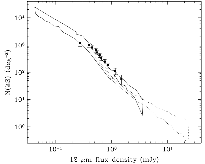
Fig. 2. Cumulative 12 \mu\text{m} galaxy counts observed with the LW10 filter from the ISO -ESS survey, plotted as full squares with error bars. The other ISOCAM 15 \mu\text{m} surveys are also plotted: the compilation by Elbaz et al. (1999) as a solid line contour, which covers the Lockman Hole (Rodighiero et al. 2004), the Marano field (Aussel et al. 1999), and the HDF North and South fields (Altieri et al. 1999) at various depths; the number-counts from the ELAIS survey (La Franca et al. 2004) are shown as a dotted line. The 15 \mu\text{m} flux densities are corrected to 12 \mu\text{m} , see text for details.
