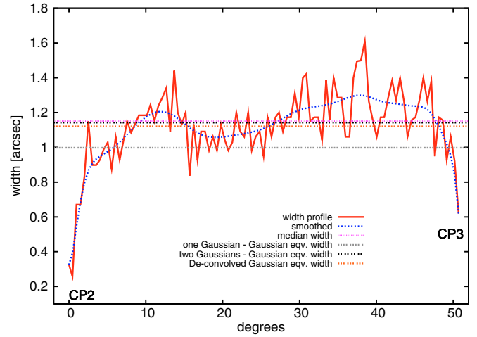
Fig. 13. Transversal width profile of arc A1 (red solid line). The blue dotted line shows an interpolation of the profile with a Bezier curve. The horizontal lines correspond to various determinations of the arc width.
