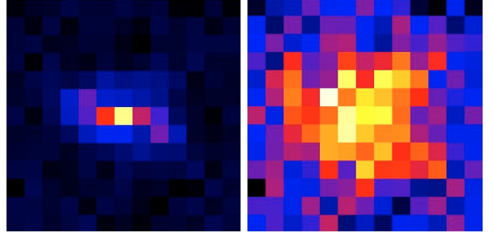
Fig. 5. The same galaxy displayed in the central panel of Fig. 3 is shown here as it should be observed in the I -band by LBT with a diffraction-limited PSF ( left panel ) and in bad seeing conditions ( \sigma = 1.2'' , right panel ). The exposure time is t_{\text{exp}} = 2000 s and the airmass is 1. The scale of each frame is 2.9'' .
