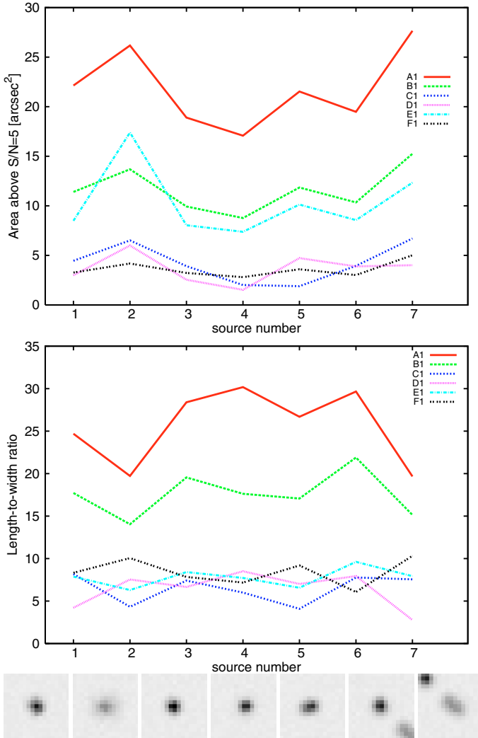
Fig. 16. Top panel: areas of the arcs A1-F1 above S/N = 5 , assuming different sets of shapelet coefficients for modeling the sources. The source models (shown in the figures below the graphs) are numbered from 1 to 7. All sources have intrinsic magnitude m_{riz} = 24 . Bottom panel: length-to-width ratio as a function of the source model.
