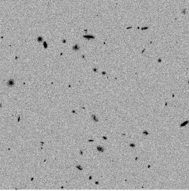
Fig. 6. Simulation of a deep field observed by HST/ACS in the z -band. The exposure time is t_{\text{exp}} = 10\,600 s and the field of view is 1' \times 1' .
