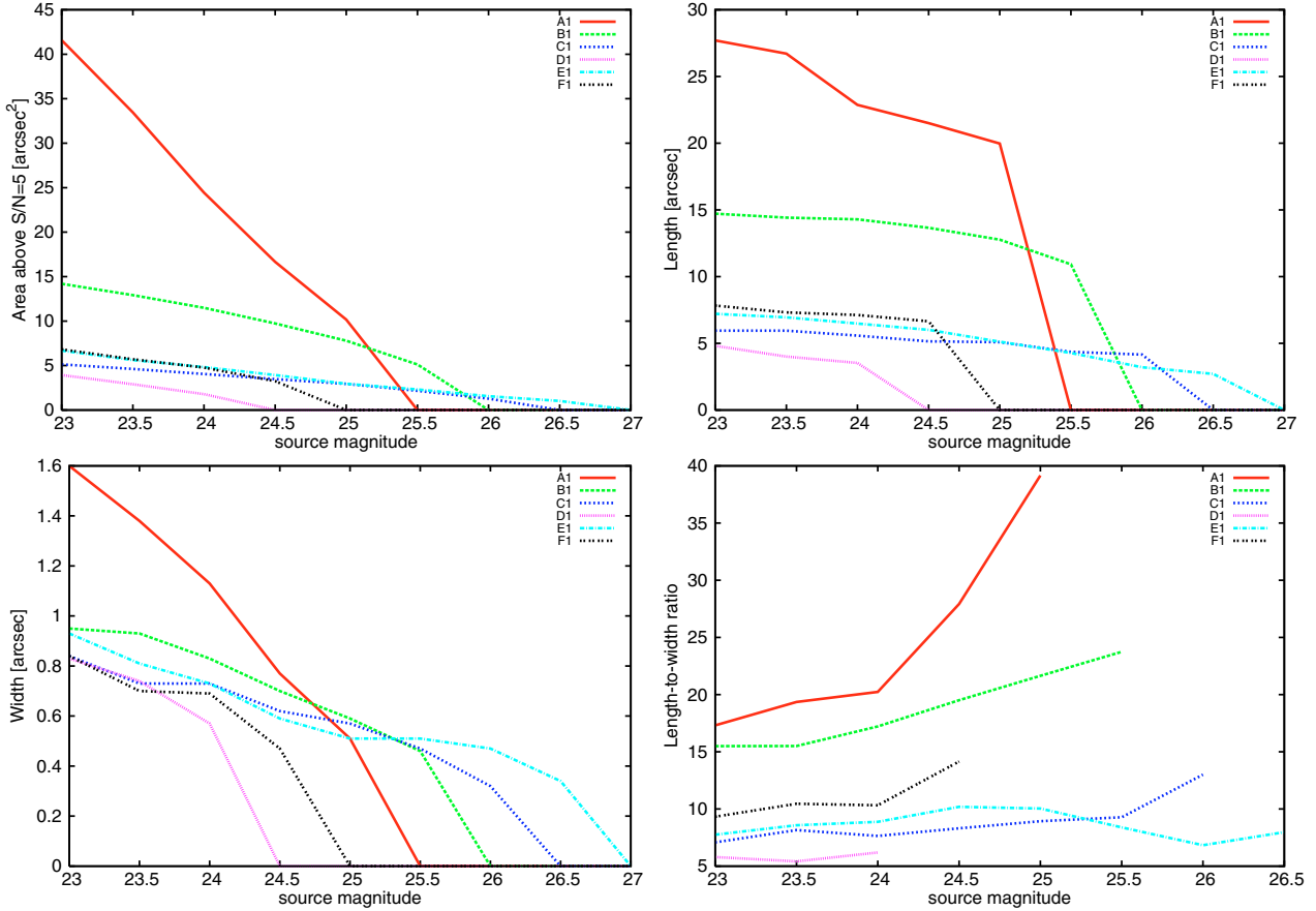
Fig. 15. Arc properties as a function of the source intrinsic magnitude in the r_{iz} band. Shown are the area above the minimal signal-to-noise ratio S/N = 5 (upper-left panel), the length (upper-right panel), the width (bottom-left), and the length-to-width ratio (bottom-right panel). The different line styles correspond to the arcs A1-F1.
