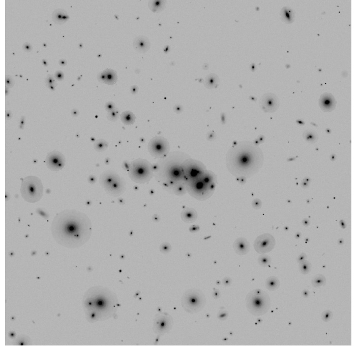
Fig. 7. Virtual observation in the z -band by HST/ACS of a galaxy cluster at z \sim 0.3 . The exposure time is t_{\text{exp}} = 1000 s and the field of view is 100'' \times 100'' . The spatial distribution and luminosities of the cluster galaxies have been obtained from semi-analytic models. The lensing effects are disabled in this simulation.
