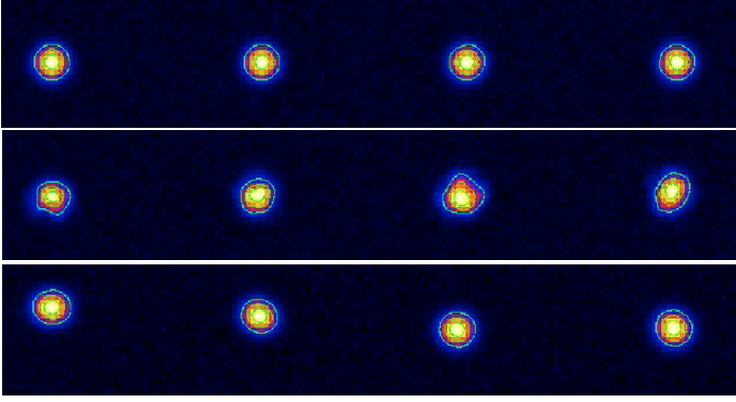
Fig. 4. Images of an array of stars observed with an LBT-like telescope. The angular separation between the stars is 10'' along the x axis. In the top panel, an isotropic PSF ( FWHM = 0.6'' ) is mimicked. In the middle panel, anisotropies varying on scales of \sim 1'' are included. In the bottom panel we simulate large-scale variations of the PSF shape on scales of \sim 15'' .
