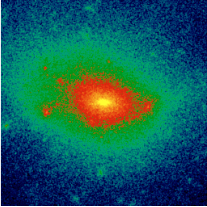
Fig. 8. Surface density map of cluster g1 corresponding to projecting the cluster along the z -axis of the simulation box. The side-length of the image is 1.5 h^{-1} Mpc comoving (corresponding to \sim 372'' ).
