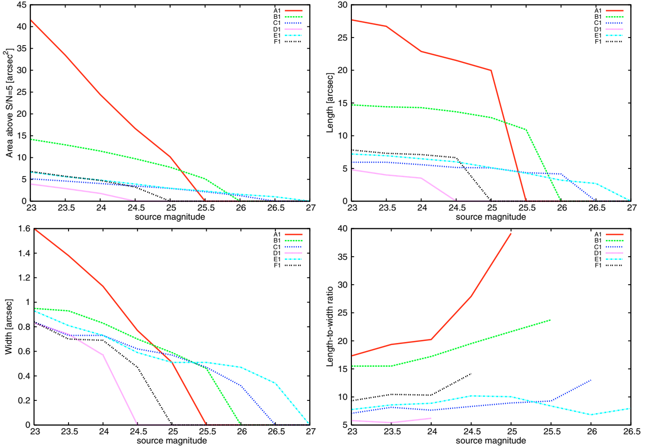
Fig. 15. Arc properties as a function of the source intrinsic magnitude in the riz band. Shown are the area above the minimal signal-to-noise ratio S/N = 5 (upper-left panel), the length (upper-right panel), the width (bottom-left), and the length-to-width ratio (bottom-right panel). The different line styles correspond to the arcs A1-F1.
