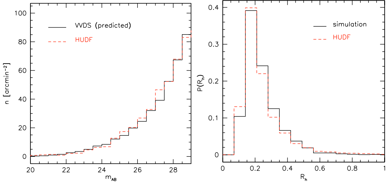
Fig. 2. Left panel: number counts per apparent magnitude bin and squared arcmin predicted by our method (solid line) and observed in the HUDF (dotted line). Magnitudes are given in the z -band. Right panel: probability distributions of the galaxy half-light radii in the HUDF (dashed histogram) and in a field simulated with Skylens (solid histogram).
