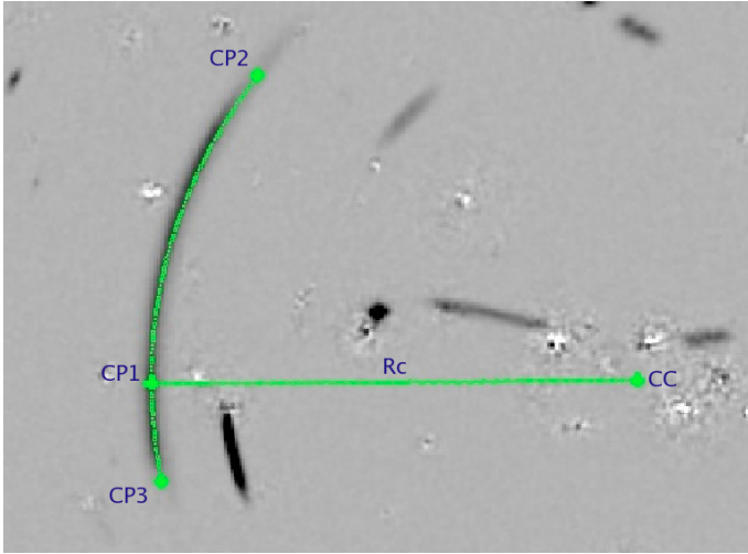
Fig. 12. Fit of the arc A1: three characteristic points have been identified on the image (CP1-3), through which a circular segment (CP2-CP3) has been traced. The curvature radius ( R_c ) and the center of curvature (CC) of the circular segment define the radius and the center of the arc.
