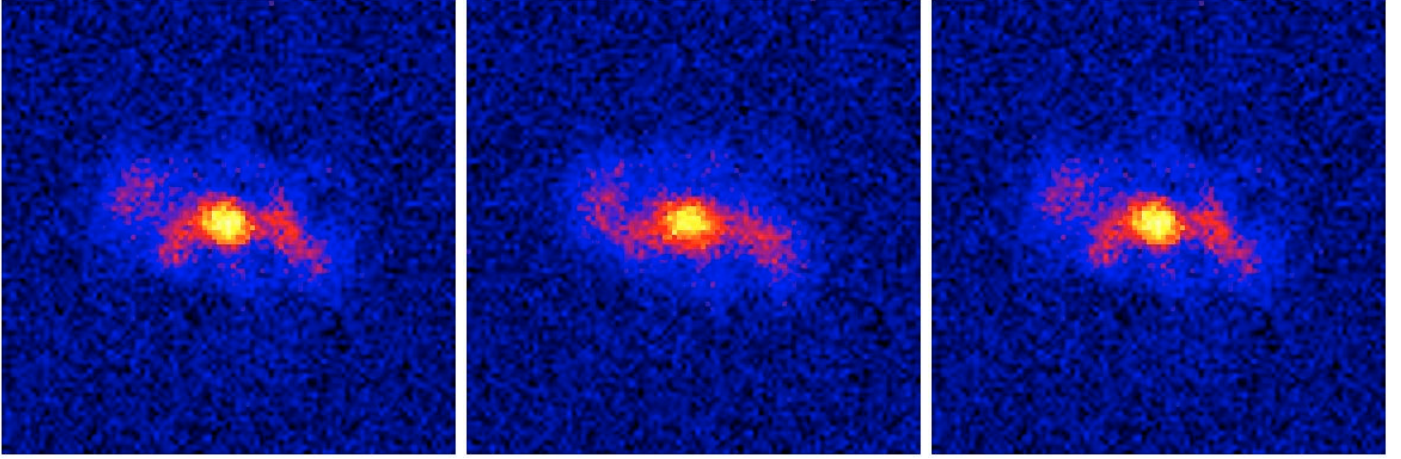
Fig. 3. Example of generation of synthetic galaxies with shapelets. In the left panel the original image of a GOODS galaxy is shown. The galaxy is decomposed into 9 \times 9 shapelets and reconstructed in the central panel . A second galaxy is then generated from the same shapelet decomposition by slightly modifying the coefficients and displayed in the right panel . The same color scale is used for all three images. To reproduce the background and the noise properties of the image in the left panel , we simulated an observation with HST/ACS (filter F850LP , t_{\text{exp}} = 10\,600 s). Each frame is 2.9'' on a side.
