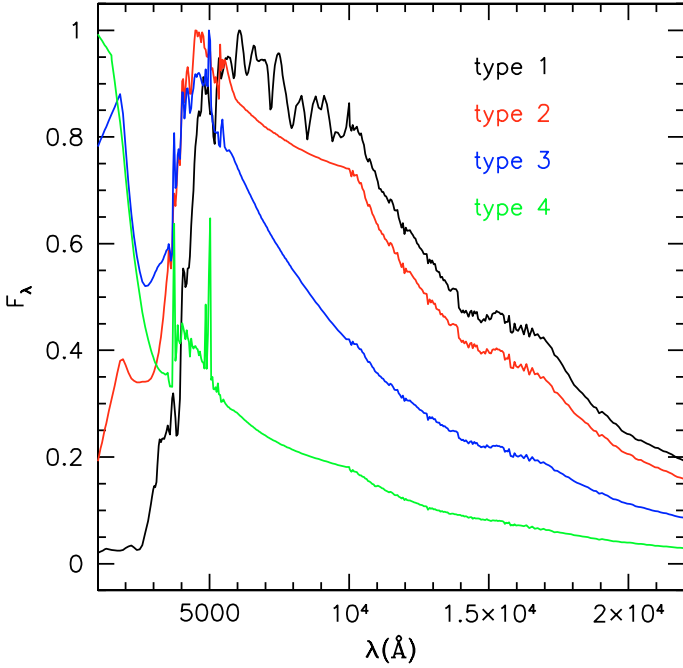
Fig. 1. Spectral-energy distributions used to characterize the galaxies of different spectral types. The galaxies are divided into four principal classes: ellipticals/S0 (type 1), early spirals (type 2), late spirals (type 3), and irregulars (type 4). The wavelengths are given in \text{\AA} , while flux is arbitrary.
