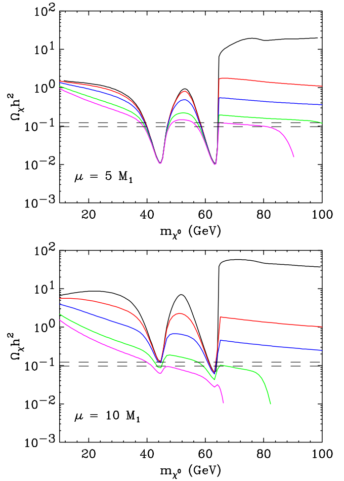
FIG. 4 (color online). The thermal neutralino relic abundance as a function of its mass for various values of the slepton masses. The slepton masses neglecting mixing are (from top to bottom) 1 TeV, 300 GeV, 200 GeV, 140 GeV, and 120 GeV. Other parameters are m_A = m_{\tilde{q}} = 1 TeV and \tan\beta = 10 . M_2 is either 2M_1 or the lowest value consistent with the LEP chargino bound, whichever is greater. The trilinear couplings A_t and A_b are selected to maximize the light Higgs mass. In the top (bottom) frame, \mu as set to 5M_1 ( 10M_1 ). The horizontal dashed lines denote the dark-matter abundance measured by WMAP [26]. The two dips correspond to the Z and light Higgs resonances.
