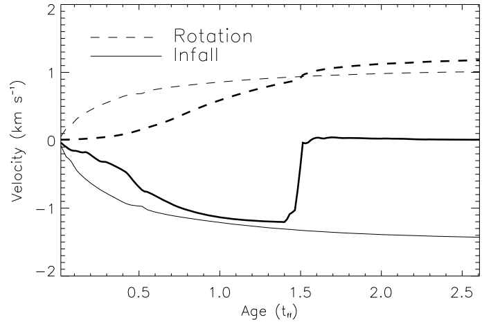
Fig. 3. The rotation and infall velocities of the collapse simulation in the mid-plane at a radius of 500 AU plotted as a function of free-fall time. The velocities of the simulation are shown in thick lines. In this figure we also show the Keplerian and free-fall velocities which are both functions of the central mass. These are shown as thin lines.
