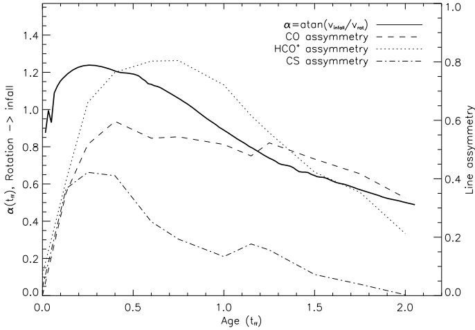
Fig. 7. The averaged \alpha from the hydrodynamical simulation plotted against free-fall time (thick solid line). The punctured lines show the dimensionless asymmetry of the single-dish spectral lines as a function of time.
