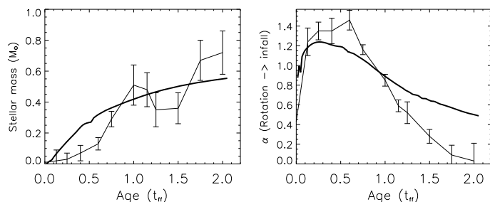
Fig. 11. High-resolution model fit, similar to that of Fig. 10. Each point shown here together with its associated error bar has been picked among the three different solutions shown in Fig. 10 using the smallest error bar as selection criterion.
