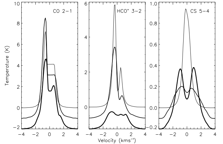
Fig. 6. Spectral line profiles of three different tracers at three different ages. t_{\text{ff}} = 1.0 and 2.0 are offset by -10\% and -20\% respectively. These spectra have been convolved with a 15'' Gaussian beam to resemble typical single-dish telescope observations.
