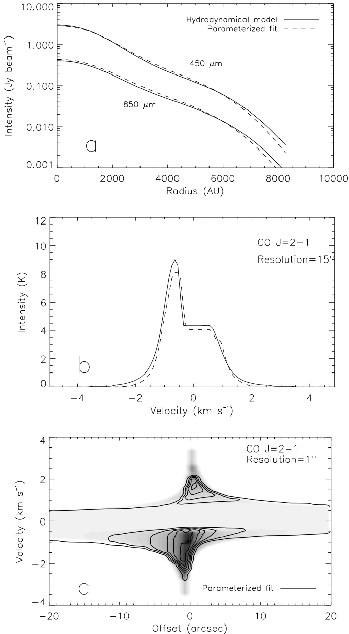
Fig. 2. Example of a fit by our parameterized model to the hydrodynamical solution at t = 1.0 t_{\text{ff}} for the case of CO. The full lines are the output of the hydrodynamical simulation and the dashed lines are the fit by our parameterized model. In panel c), the hydrodynamical output is shown by the gray scale and the model fit by contour lines.
