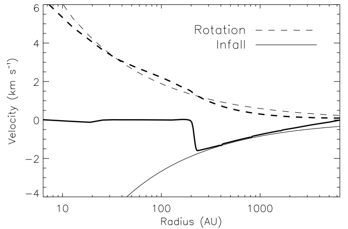
Fig. 4. The rotation and infall velocities in the simulation along the mid-plane at an age of t = 1.0 t_{\text{ff}} . As in Fig. 3, the thin lines correspond to free-fall and Keplerian velocity profiles.
