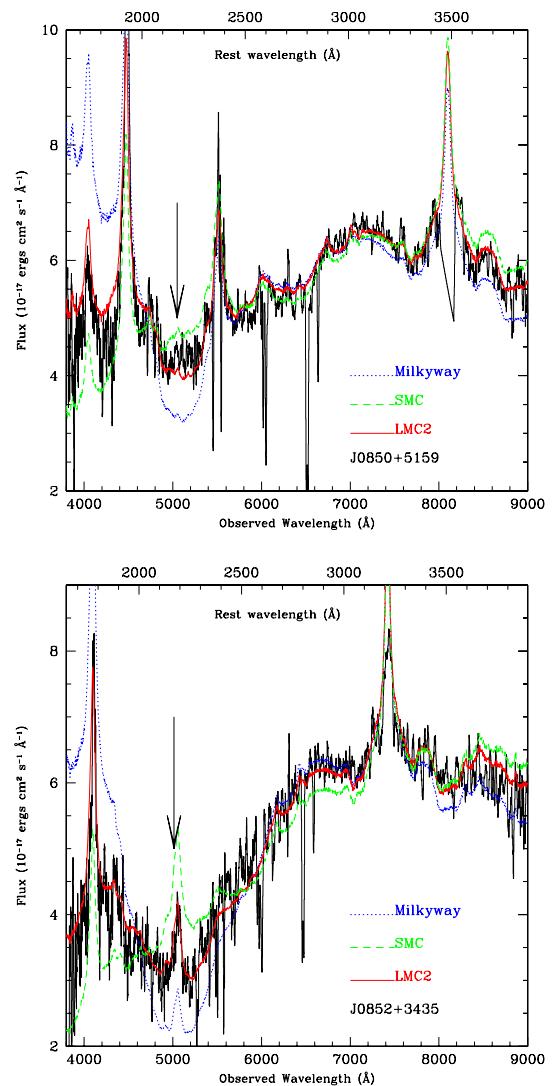
Figure 2. The SDSS spectrum of J0850+5159 (top panel) and J0852+3435 (bottom panel) is fitted with SDSS composite spectrum corrected using average extinction curves from the Milky Way (dotted line), the LMC2 Supershell (solid line) and the SMC (dashed line). Rest wavelengths at z_{\text{abs}} are indicated at the top of the figure. The arrow marks the location of 2175 \text{\AA} feature at z_{\text{abs}} . For presentation purpose, the observed spectrum is boxcar smoothed by 10 pixels.
