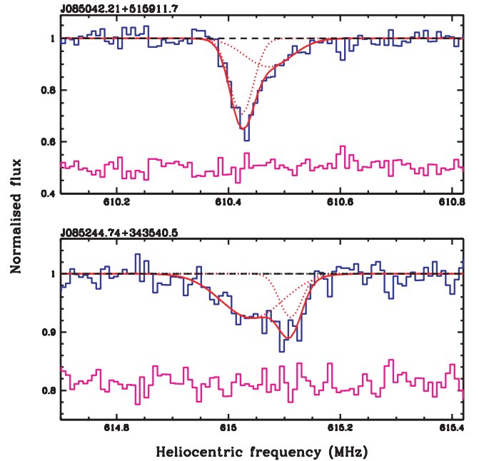
Figure 1. GMRT spectra of J085042.21+515911.7 (top panel) and J085244.74+343540.5 (bottom panel). H I 21-cm absorption is detected at z_{\text{abs}} = 1.3265 and 1.3095 (see Table 2), respectively. The solid lines represent the fits to the overall profiles. Individual Gaussian components are shown with dotted lines. Residuals, on a scale arbitrarily shifted for clarity, are also plotted.
