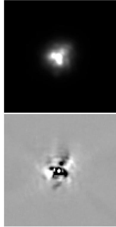
Fig. 11. Images of HD 17156. Upper panel : image of HD 17156 obtained with the AdOpt module of TNG. A similar quasi-static speckle pattern can be seen. Lower panel : difference between two images taken with two different field orientations, which allows us to significantly improve detection limits in the inner regions. The field of view shown is 4.3 \times 4.3'' . The images are displayed in linear gray scale.
