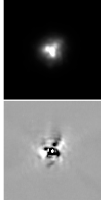
Fig. 11. Images of HD 17156. Upper panel: image of HD 17156 obtained with the AdOpt module of TNG. A similar quasi-static speckle pattern can be seen. Lower panel: difference between two images taken with two different field orientations, which allows us to significantly improve detection limits in the inner regions. The field of view shown is 4.3 × 4.3". The images are displayed in linear gray scale.
