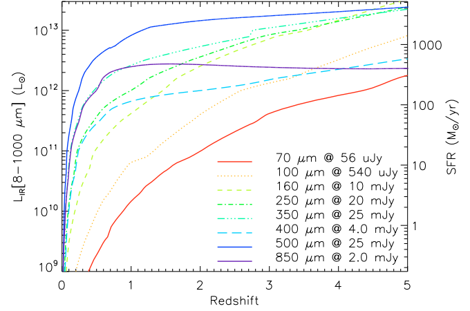
Fig. C.2. Detection limits for confusion limited surveys from 70 to 850\ \mu\text{m} . The curves show the minimum IR luminosity ( 8 – 1000\ \mu\text{m} ), or equivalently SFR ( =L_{\text{IR}} \times 1.72 \times 10^{-10} ), that can be detected for a star-forming galaxy assuming that it has an SED similar to the Chary & Elbaz (2001) ones. The 70 , 100 , 160 , 250 , 350 and 500\ \mu\text{m} limits correspond to a 3.5 m telescope diameter, such as Herschel or SPICA, while the 400\ \mu\text{m} is for a 12 m class telescope such as APEX (e.g. ARTEMIS, we show the average between the two bands at 350 or 450\ \mu\text{m} to avoid confusion with Herschel) and the 850\ \mu\text{m} is for a 15 m telescope as the JCMT (SCUBA).
