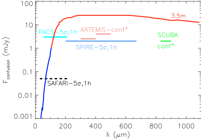
Fig. C.1. Confusion limit for a 3.5 m telescope. The 5\sigma -1 h limits of SPICA-SAFARI ( 50\ \mu\text{Jy} , 33 – 210\ \mu\text{m} , dashed line), Herschel PACS ( 3\ \text{mJy} , 55 – 210\ \mu\text{m} , light blue line) and SPIRE ( 2\ \text{mJy} , 200 – 670\ \mu\text{m} , blue line) are shown together with their wavelength ranges. The blue part of the curve is determined by the source density criterion (i.e. the requirement to have less than 30% of the sources closer than 0.8 \times FWHM ), the red part is defined by the photometric criterion, i.e. sources must be brighter than 5 times the rms due to very faint sources below the detection limit.
