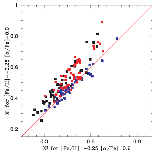
Figure 5. The reduced \chi^2 of a composite age fit to the spectra of a sample of 150 early-type galaxies from the SDSS at fixed [Fe/H] = -0.25 and [\alpha/\text{Fe}] = 0.2 (abscissa) and [\alpha/\text{Fe}] = 0.0 (ordinate). Objects are split by mass, with the lowest in blue, intermediate in black and high-mass objects in red.
