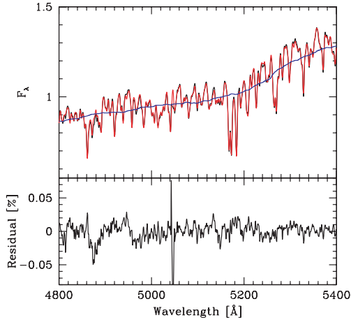
Figure 2. The spectrum of NGC 6528 (black), labelled as a_2 , as taken from Schiavon et al. (2005) and the best-fitting model from PegHR+C07 (red). The blue line is the continuum that was used to normalize the observed spectrum. The model was fit to the data only in the wavelength range 4828–5364 Å.
