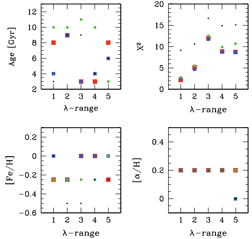
Figure 3. The dependence of the best-fitting parameters on the wavelength range that was used for the fit and on the model. The numbers of the wavelength ranges are given in the text of Section 4. We show results for one spectrum (NGC 6528/_a/_2) and for all models, i.e. V09+C07 (red), PegHR+C07 (blue), BC03+C07 (green) and C07 (black).
