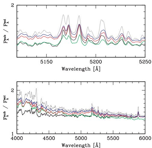
Figure 1. The ratios between SSPs of 10Gyr at subsolar metallicity ( Z = 0.005 , [\text{Fe}/\text{H}] = -0.5 , [\alpha/\text{Fe}] = 0 ) and solar metallicity ( [\text{Fe}/\text{H}] = 0 , [\alpha/\text{Fe}] = 0 ) for different stellar population models (black C07, green BC03, blue PegHR and red V09). The dotted line is C07 at the same Z = 0.005 , but different abundance ratios ( [\text{Fe}/\text{H}] = -0.85 and [\alpha/\text{Fe}] = 0.4 ). All models have been smoothed to a common resolution of \sigma = 1 Å in the upper panel and \sigma = 5 Å in the lower panel.
