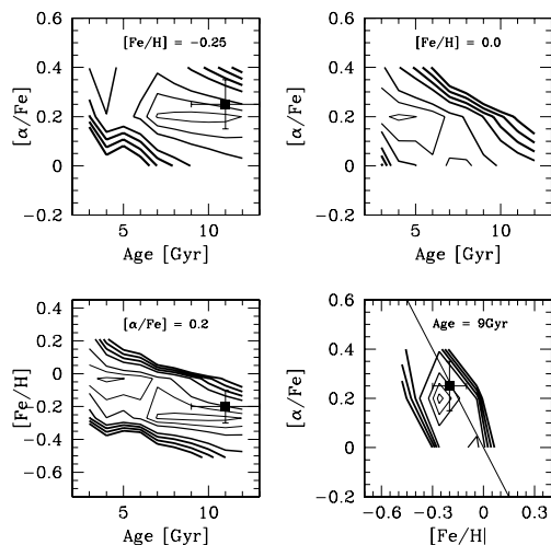
Figure 4. The distribution of \chi^2 for the NGC 6553_1 spectrum and determined over the wavelength region 4828–5364 Å, depending on the SSP parameters age, [Fe/H] and [\alpha/\text{Fe}] using the V09+C07 model. The thicker the line, the higher the value of \chi^2 , in steps of \Delta\chi^2 = 1 . The squares with error bars show the literature values from Table 1. The upper-right panel shows that it is important to obtain both [Fe/H] and [\alpha/\text{Fe}] correctly, in order to avoid a biased age measurement. In the lower-right panel, the locus of constant total metallicity Z = 0.017 is indicated by a thin straight line.
