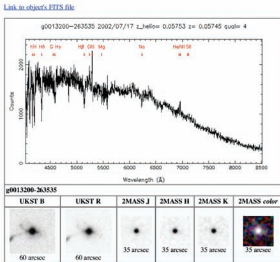
Figure 5. Example spectroscopic and photometric frames from the 6dFGS online data base for (a) a nearby bright galaxy at z = 0.057 ( Q = 4 ) from the K -selected sample (PROGID = 1), and (b) a candidate double QSO at z = 2.524 ( Q = 2 ) from the Hamburg-ESO QSO sample (PROGID = 129). 2MASS and UKST frames are only available for sources selected as part of the original 6dFGS primary samples, where available in one or more of KHRrFbJ .
