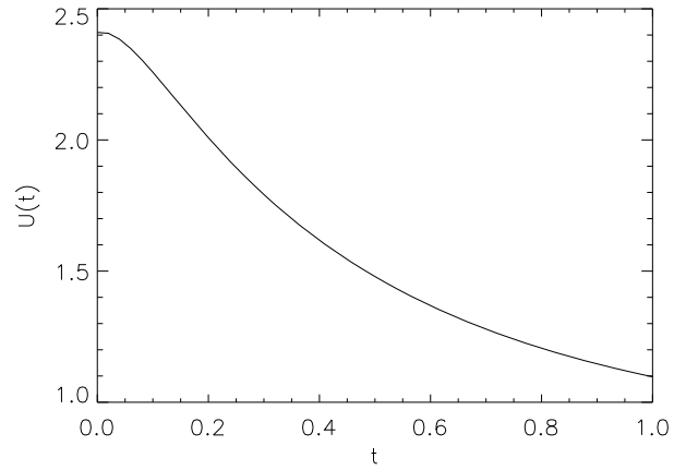
Fig. 3. Evolution of the reduced iron volume emissivity in the iron helium-like lines in the region with a temperature of 10.0 keV. The dimensionless time is given by t/(3 \times 10^7 \text{ yr}) .
