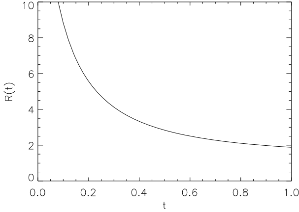
Fig. 5. Evolution of the iron line flux ratio in the region with a temperature of 10.0 keV. The dimensionless time is given by t/(3 \times 10^7 \text{ yr}) .
