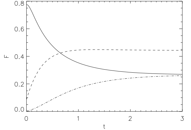
Fig. 4. Dependence of the He-like (solid line), H-like (dashed line) and fully ionized (dot-dashed line) ionic fractions of iron on the dimensionless time t/(3 \times 10^7 yr).
