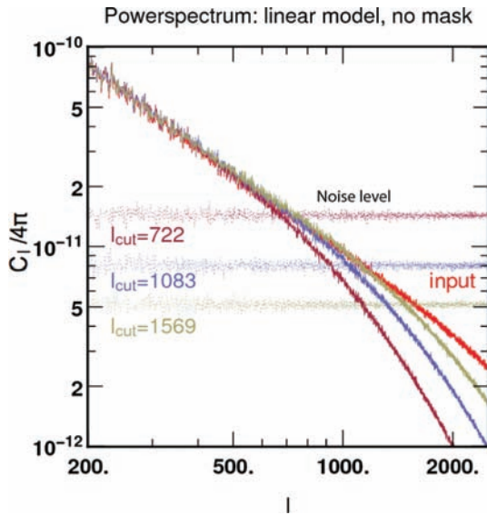
Figure 6. A zoom on the power spectra of the three reconstructions of 2048 S_{\text{FS}}^{\ell_{\text{cut}}} for \ell_{\text{cut}} = 722, 1083 and 1569 (respectively 24, 44 and 78 ngal/□ arcmin), together with the power spectra of the noise. Note that the level of smoothing decreases with increasing S/N, in parallel to the bias in the corresponding power spectrum.
