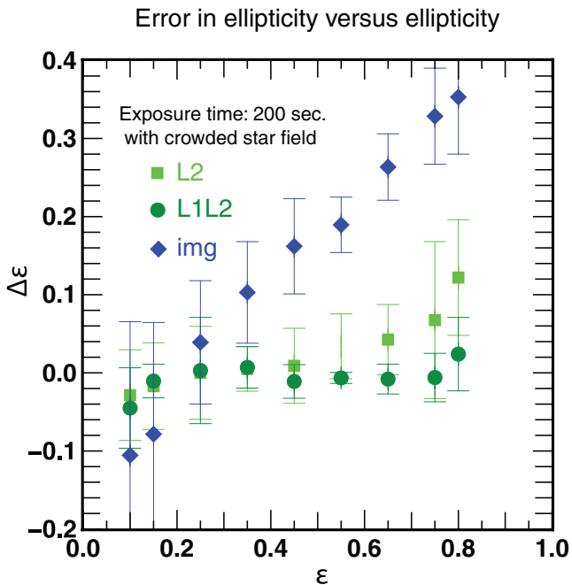
Figure 3. The error in ellipticity as a function of the ellipticity (measured by SExtractor) for a set of 50 images (such as those shown in Fig. 2) either directly on the image (medium diamonds), deconvolved with \ell_2 gradient penalty function with enforced positivity (light squares) and \ell_1 - \ell_2 gradient penalty function with positivity (dark circles). For each set, the ellipticity is also measured directly on the raw image. Note that, as expected, the error on the bias is largest for circular galaxies, since deconvolution will tend to overamplify departure from circular symmetry.
