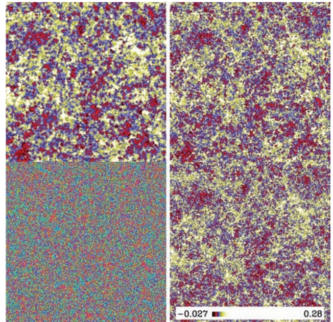
Figure 18. A zoom of the full-sky recovered \kappa maps of a simulation _{2048}S_{FS}^{\ell_{\text{cut}}} with \ell_{\text{cut}} = 722 (top-left panel) and 1569 (top-right panel) (respectively 24 and 78 \text{ngal}/\square \text{ arcmin} ) at coordinates (\phi, \theta) = (0, 0) (the colour table corresponds to a histogram equalization); bottom-left panel: the corresponding data (the hue colour table codes the shear orientation); bottom-right panel: the corresponding underlying \kappa map.
