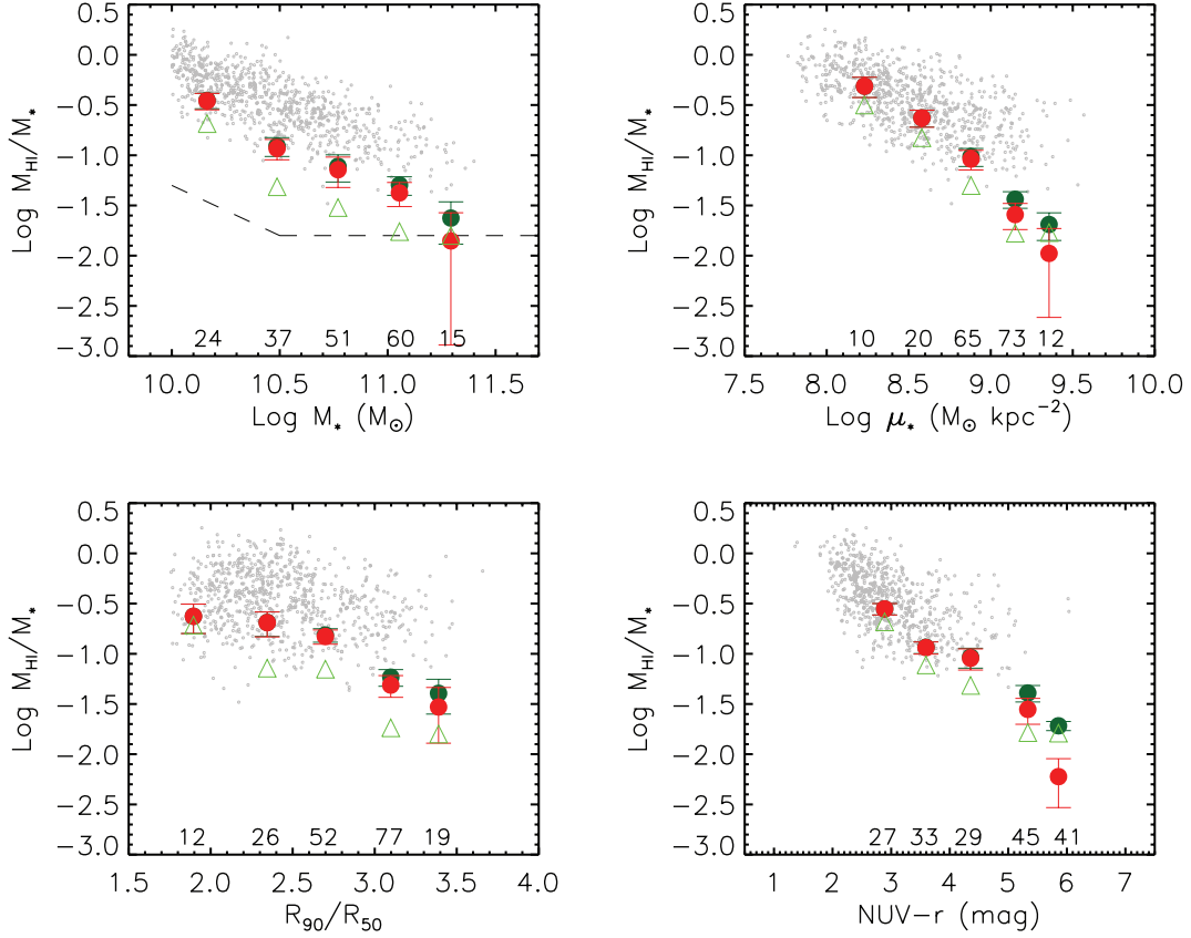
Figure 9. Average trends of H I mass fraction as a function of stellar mass, stellar mass surface density, concentration index and observed NUV– r colour based on the representative sample discussed in Section 7.2. In each panel, large circles indicate average gas fractions (weighted as explained in the text). These were computed including the non-detections, whose H I mass was set to either its upper limit (dark green) or zero (red). Green triangles are weighted medians. The average number of galaxies in each bin, N_i , is indicated above the x -axis; only bins with N_i \geq 8 are shown. These results are listed in Table 4. Galaxies in the GASS parent sample detected by ALFALFA are plotted as small grey circles. The dashed line in the first panel shows the H I detection limit of GASS.
