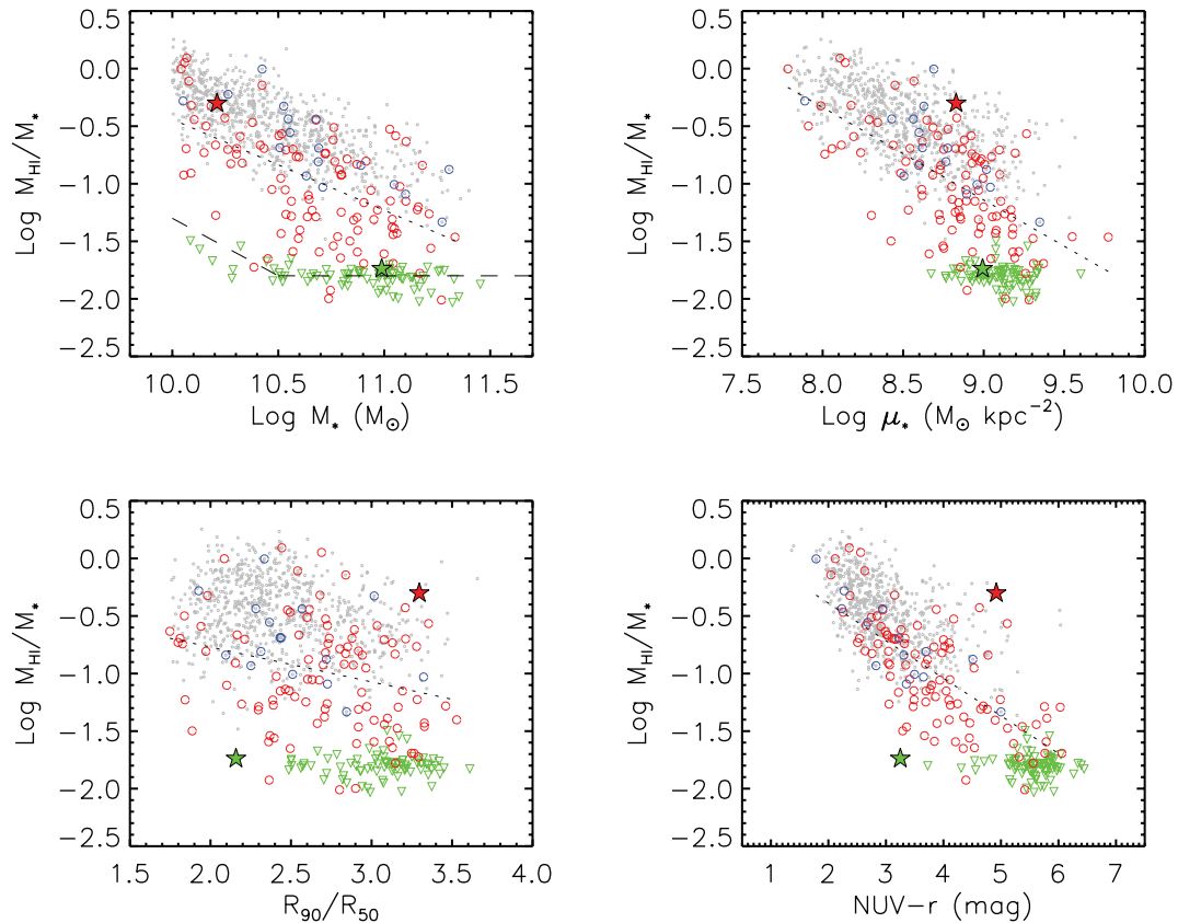
Figure 8. The H I mass fraction of the GASS sample is plotted here as a function of stellar mass, stellar mass surface density, concentration index and observed NUV - r colour. Red circles and green triangles represent detections and non-detections, respectively. Blue symbols indicate randomly selected, H I-rich ALFALFA and S05 galaxies added to the DR1 sample in the correct proportion, to compensate for the fact that we do not re-observe objects with good detections in either of those archives. The sample including red, green and blue symbols is one example of the catalogues described in Section 7.2, and contains 193 galaxies. For comparison, we also show the full set of ALFALFA galaxies meeting the GASS selection criteria that have been catalogued to date (grey). The stars in all plots highlight the locations of two interesting objects, GASS 3505 (red) and GASS 7050 (green), discussed in the text. The dashed line on the top left-hand panel indicates the H I detection limit of GASS. Dotted lines in each panel are linear fits to the red and blue circles only.
