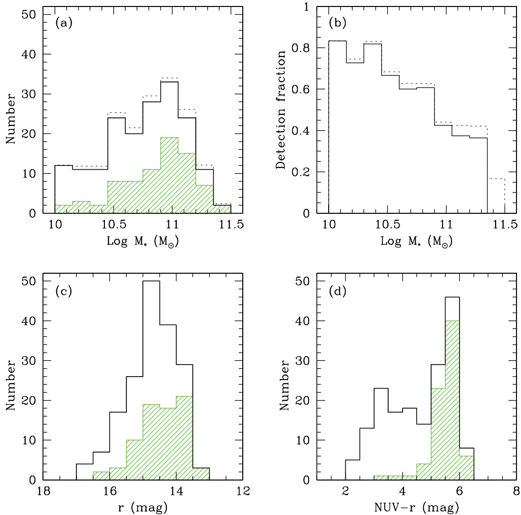
Figure 7. Stellar mass (a), SDSS r -band (c) and observed NUV– r colour (d) distributions for the GASS DR1 sample (solid). Hatched histograms indicate the corresponding distributions for the non-detections. The detection fraction (i.e. the ratio of detections to total) is shown as a function of stellar mass in (b). The dotted histograms in the top panels are the average distributions for the representative sample discussed in the text (Section 7.2).
