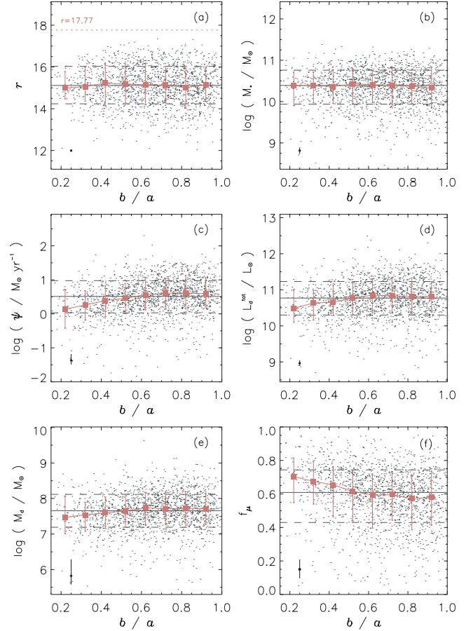
Figure 9. Galaxy properties plotted against the ratio of minor to major axes b/a (used as a proxy for inclination) for the 1658 galaxies with highest S/N photometry in the matched GALEX –SDSS–2MASS–IRAS sample described in Section 2: (a) apparent r -band magnitude, r ; (b) stellar mass, M_* ; (c) star formation rate averaged over the last 10^8 yr, \psi ; (d) total infrared luminosity, L_d^{\text{tot}} ; (e) dust mass, M_d ; (f) fraction of L_d^{\text{tot}} contributed by dust in the diffuse ISM, f_\mu . Red squares and error bars indicate the median values and 16th–84th percentile ranges in bins of b/a . For reference, the horizontal solid and dashed grey lines indicate the median value and 16th–84th percentile range for the whole sample (i.e. including all inclinations). The median observational error in r is indicated in the lower-left corner of panel (a). In each panel from (b) to (f), the median confidence interval in the likelihood estimates of the considered parameter is indicated in the lower-left corner.
