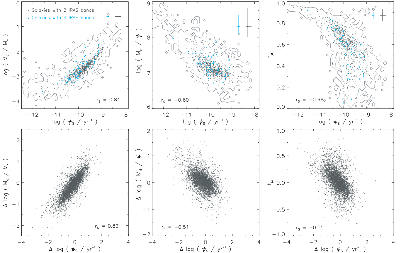
Figure 6. Top: median-likelihood estimates of three galaxy properties against specific star formation rate, \psi_s . Left-hand panel: ratio of dust mass to stellar mass, M_d/M_* . Middle panel: ratio of dust mass to star formation rate, M_d/\psi (which may be used as a proxy for the dust-to-gas ratio; see Section 4). Right-hand panel: fraction of total infrared luminosity contributed by dust in the ambient ISM, f_\mu . In each panel, the grey contour shows the distribution of the full matched GALEX –SDSS–2MASS–IRAS sample described in Section 2, while the points show the distribution of the subsample of 1658 galaxies with highest S/N photometry in all bands. The blue triangles show galaxies with complete IRAS information in the 12-, 25-, 60- and 100- \mu\text{m} bands. The error bars represent the median confidence ranges in each parameter. Bottom: differences in the same quantities as in the top panels for pairs of galaxies closely matched in stellar mass (see text for detail). The Spearman rank coefficient r_s is indicated in each panel.
