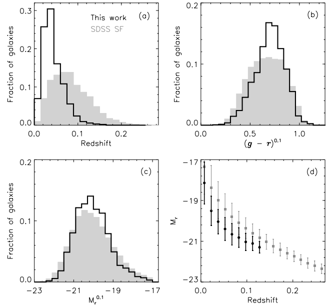
Figure 2. Properties of the SDSS DR6 star-forming galaxies (in grey) and the matched GALEX –SDSS–2MASS– IRAS subsample considered in this work (in black). The histograms show the normalized distributions of the following parameters: (a) redshift, z ; (b) Galaxy g - r colour, k -corrected to redshift z = 0.1 ; (c) absolute r -band model magnitude, k -corrected to redshift z = 0.1 , M_r^{0.1} . Panel (d) shows the mean r -band absolute magnitude, M_r , in different redshift bins for both samples (the error bars represent the standard deviation \pm \sigma in each bin).
