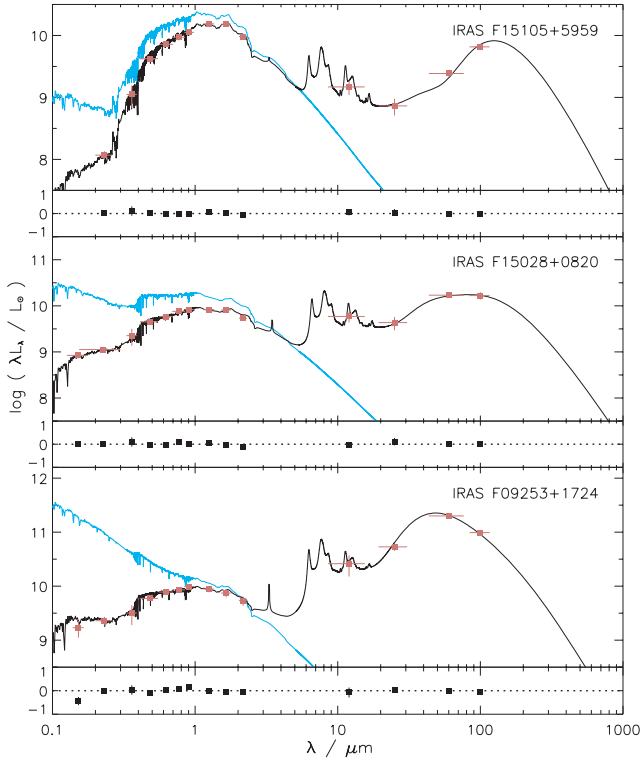
Figure 4. Best-fitting models (in black) to the observed spectral energy distributions (in red) of three galaxies spanning wide ranges in star formation and dust properties in the matched GALEX – SDSS – 2MASS – IRAS sample described in Section 2: from quiescent, moderately dusty (top panel) to actively star-forming, highly dusty (bottom panel). In each panel, the blue line shows the unattenuated stellar spectrum. The red squares show the observed broad-band luminosities ( GALEX FUV, NUV; SDSS ugriz ; 2MASS JHK s ; IRAS 12, 25, 60 and 100 \mu\text{m} ) with their errors as vertical bars and the widths of the filters as horizontal bars. The fit residuals ( L_{\lambda}^{\text{obs}} - L_{\lambda}^{\text{mod}}/L_{\lambda}^{\text{obs}} ) are shown at the bottom of each panel.
