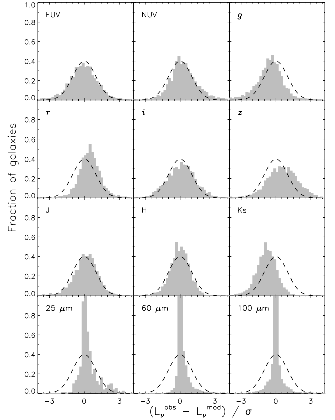
Figure 3. Distribution of the difference between observed luminosity L_v^{\text{obs}} and best-fitting model luminosity L_v^{\text{mod}} , in units of the observational error \sigma , for the galaxies in the matched GALEX –SDSS–2MASS– IRAS sample described in Section 2. Each panel refers to a different photometric band, as indicated. For reference, the black dashed curve shows a Gaussian distribution with unit standard deviation. The best-fitting model for each galaxy was selected by fitting as many fluxes as available in the following bands: GALEX (FUV and NUV), SDSS ( ugriz ), 2MASS ( JHK s ) and IRAS (12, 25, 60 and 100 \mu\text{m} ).
