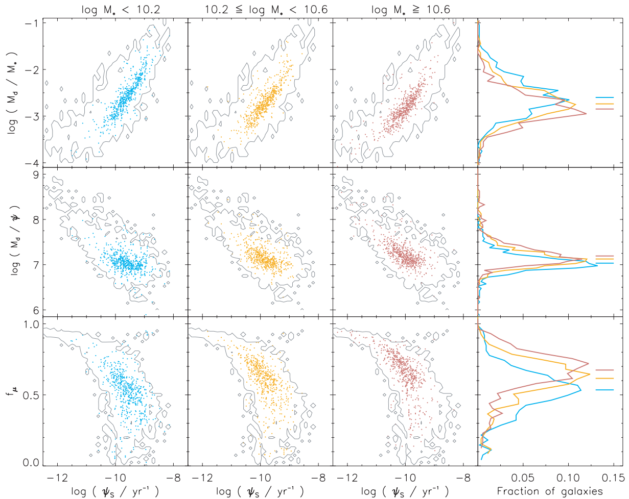
Figure 7. Same relations as in the top panels of Fig. 6 plotted in three stellar-mass ranges: \log(M_*/M_\odot) < 10.2 (blue); 10.2 \leq \log(M_*/M_\odot) < 10.6 (orange); \log(M_*/M_\odot) \geq 10.6 (red). The right-hand panels show the corresponding distributions of the dust-to-stellar mass ratio M_d/M_* , the ratio of dust mass to star formation rate M_d/\psi and the fraction f_\mu of total infrared luminosity contributed by dust in the ambient ISM, along with their median values. The contours are the same as in the top panels of Fig. 6.
