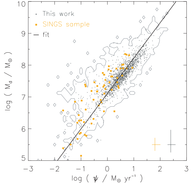
Figure 5. Median-likelihood estimate of the dust mass, M_d , versus that of the star formation rate averaged over the last 10^8 yr, \psi , for the matched GALEX – SDSS – 2MASS – IRAS sample described in Section 2 (in grey) and the SINGS galaxies (in orange). The grey contour shows the distribution of the full matched sample of 3258 galaxies, while grey points show the distribution of the subsample of 1658 galaxies with highest S/N photometry in all bands (see text). The median error bars for each sample are indicated in the lower-right corner. These correspond to the median 16th–84th percentile range of the likelihood distributions in M_d and \psi . The black line shows a linear fit to the grey points, computed as the bisector of the least-square regression lines on each axis.
