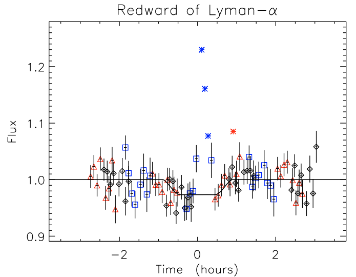
Fig. 9. Plot of the flux redward of Lyman- \alpha . The time has been phase-folded and the flux normalized by the linear baseline shown in Fig. 8. Outliers at 3\text{-}\sigma are plotted with stars.
