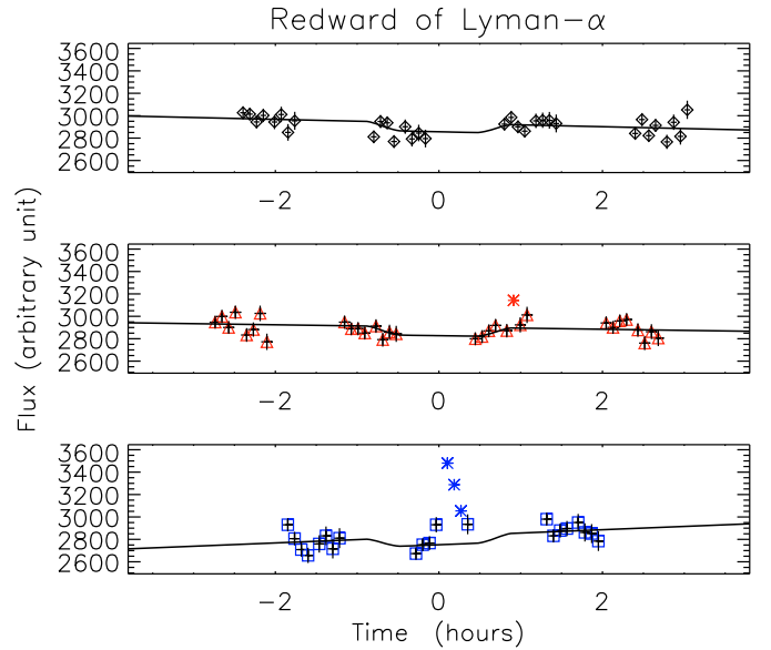
Fig. 8. Plot of the flux redward of Lyman- \alpha for the three HST transits. Some measurements are clearly outliers; measurements beyond 3\text{-}\sigma from the best fit are plotted with stars. Symbols are the same as in Fig. 4
