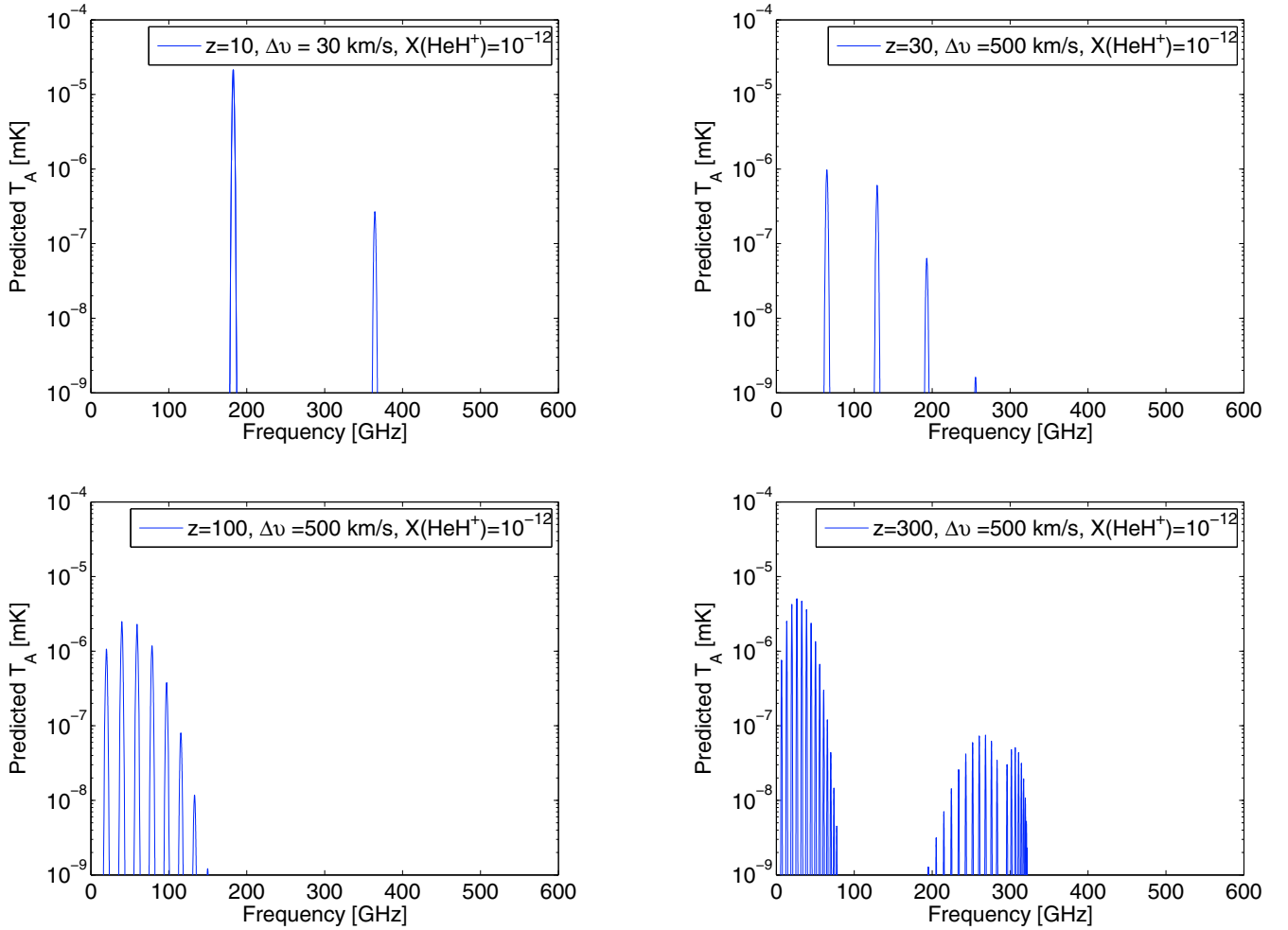
Fig. 6. These plots are an example with the main goal to give an idea of the pattern of the primordial spectral lines: predicted antenna temperature \Delta T_A^* of resonant HeH + optically thin lines within the 2:1 Odin beam at z = 10, 30, 100, and 300 . Turn-around phase is assumed for z = 10 and for higher z we assume linear phase with line widths as indicated in the legends. We also assume a low density n_H = 2 \times 10^{-7} (1+z)^3 and X(\text{HeH}^+) = 10^{-12} . Note, that any increase of the density, abundance, or decrease of line width, directly increases the amplitude of the signals with an equal magnitude. If thermal absorption processes are present, they may be several orders of magnitudes stronger than the resonant lines. The amplitudes of the ro-vibrational lines are lower than 10^{-8} mK until z \sim 300 , when they show up around 200 to 300 GHz. They are, however, orders of magnitudes weaker than the rotational lines.
