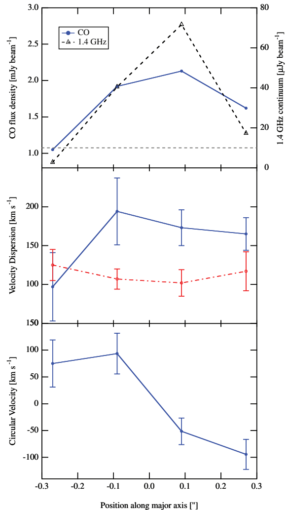
Figure 4. Kinematic analysis for HDF 132 (SMM J123618.33+621550.5). Spectra were taken at points along the major axis of the galaxy with \sim 0.15 \text{ arcsec} spacing ( \simeq 1/3 – 1/2 of the beam FWHM), and resultant kinematic parameters were derived. Bottom panel: circular velocity; as the CO spectrum for HDF 254 is double peaked, the velocity was obtained by taking the mean of the two peaks, with the weighting of each component taken as the height of the respective peak. Middle panel: velocity dispersion, obtained via the width of the same Gaussian peak. The solid blue line shows the blueshifted peak, whereas the dashed red line shows the redshifted peak. Top panel: CO surface brightness (blue solid line). For reference, the MERLIN-obtained 1.4 GHz continuum flux density measured at the same points has been overlaid (black dashed line and right-hand axis). The dashed horizontal line is drawn at 10 \mu\text{Jy beam}^{-1} (approximately three times the image rms).
