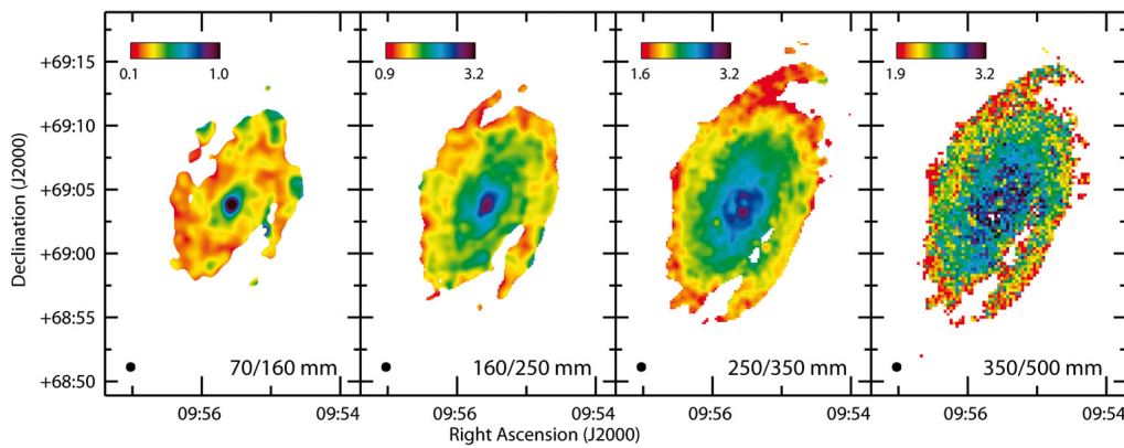
Fig. 2. Images of the 70/160, 160/250, 250/350, and 350/500 \mu\text{m} surface brightness ratios in the optical disc of M81. Each image is created using data with PSFs that match the 500 \mu\text{m} PSF. Regions not detected at the 3\sigma level in the two bands used for each ratio are left blank. The image sizes and orientations are the same as for Fig. 1. The circles in the lower left corner of each image show the FWHM of the 500 \mu\text{m} PSF.
