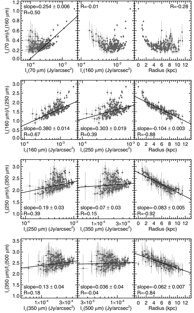
Fig. 3. The 70/160 , 160/250 , 250/350 , and 350/500\ \mu\text{m} surface brightness ratios versus the surface brightness ( left and center ) and inclination-corrected galactocentric radius ( right ). The data were measured in 42'' subregions in images with PSFs that matched the PSF of the 500\ \mu\text{m} data. Best fit lines are shown for all plotted data except for two relations involving the 70/160\ \mu\text{m} ratio, where the fits were very poor; corresponding slopes are given in the panels. The R values are the Pearson correlation coefficients for the plotted data. Note that, in the left-side and center panels, the logarithm of the surface brightnesses are used for the best fit lines and correlation coefficients.
