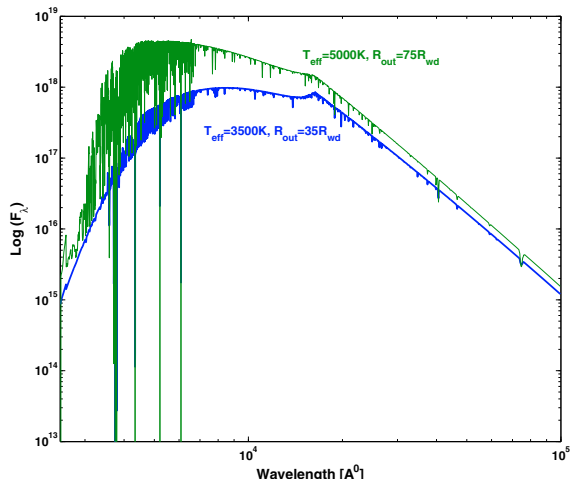
Fig. 15. The integrated disc spectrum for two low values of T_{\text{eff}} = 5000 and 3500 ( M_{\text{wd}} = 0.6 M_{\odot} , \alpha = 0.03 ).
