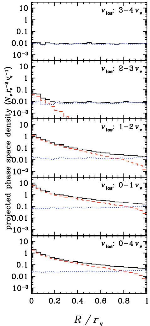
Fig. 5. Phase space density of stacked virial cone as a function of projected radius in bins of absolute line-of-sight velocities (marked on the upper-right of each plot). Dashed (red) and dotted (blue) histograms represent the halo particles ( r < r_v ) and the interlopers ( r > r_v ), respectively, while the solid histograms (artificially moved up by 0.06 dex for clarity) represent the full set of particles. There are no halo particles at v > 3v_v (top plot).
